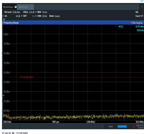
Band7-15MHz-QPSK-20825-1RB#74-0.15~30-P
