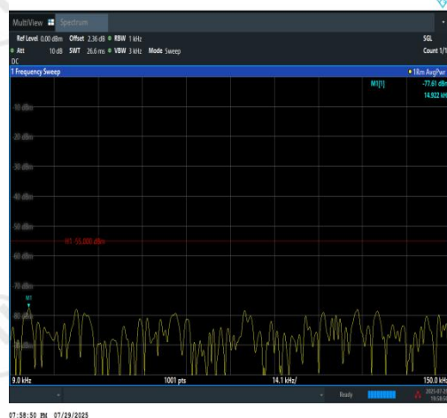
Band7-15MHz-16QAM-20825-75RB#0-0.009~0.15 15-PASS
