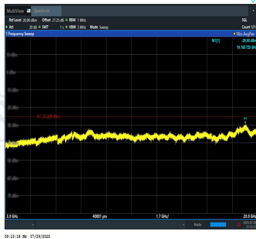
Band7-15MHz-16QAM-20825-1RB#74-3000~20 000-PASS
