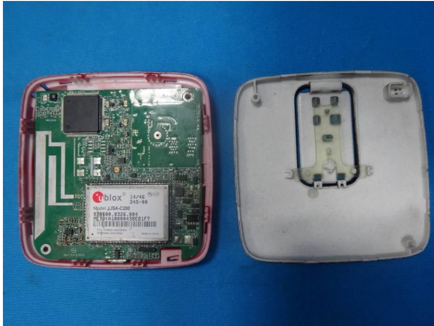
EUT Internal: Front panel removed
