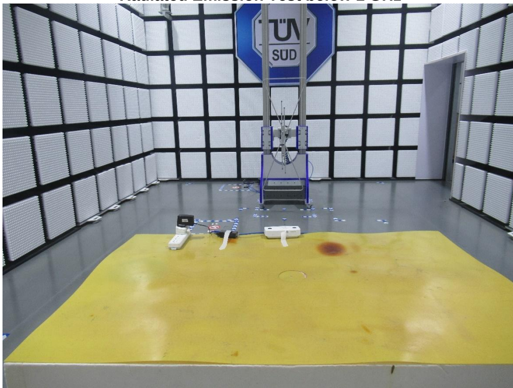
Radiated Emission Test below 1 GHz
