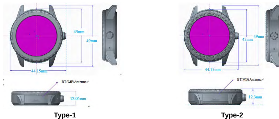
Fig.7 Antenna location
