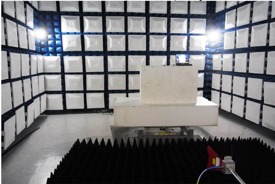
Radiated Emission (above 1GHz) Set up Photo
