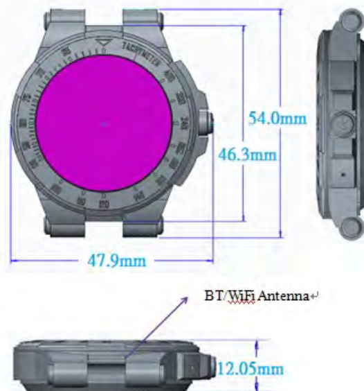
Fig.6 Antenna location
