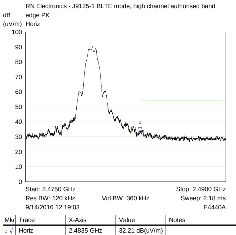
Upper Authorised Band Edge Plot
