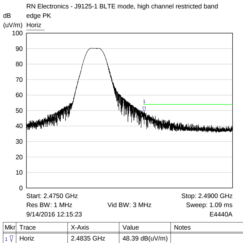
Upper Restricted band edge Peak Plot
