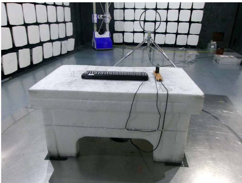
Radiated H-Field Emissions (150 kHz to 30 MHz)
