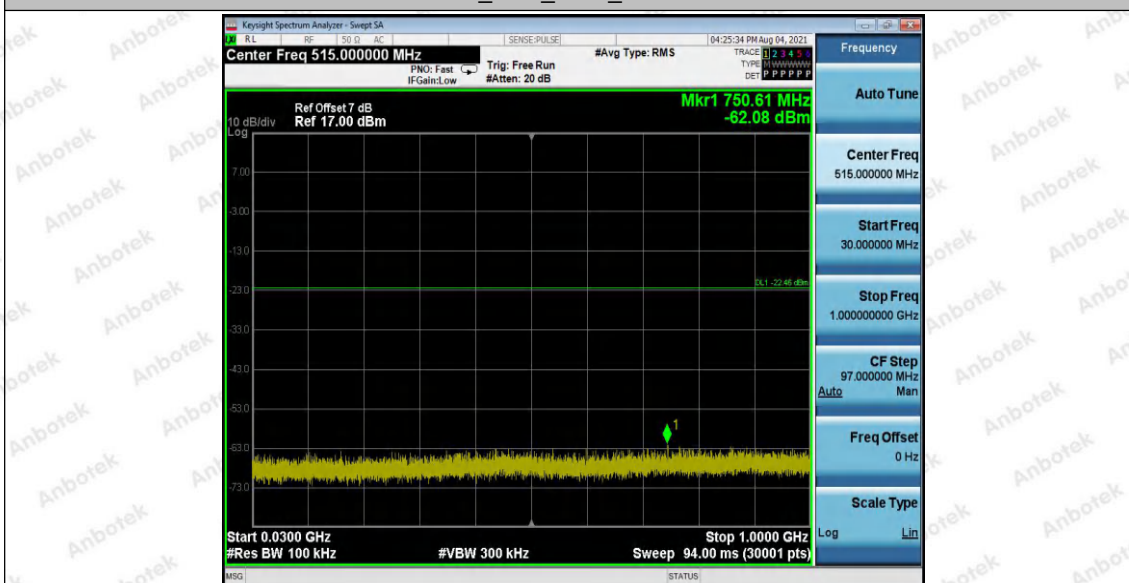
DH5_Ant1_2441_30~1000
