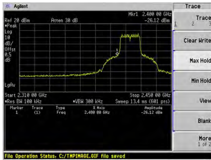
802.11n-20 MHz LOW CHANNEL, Reference level
