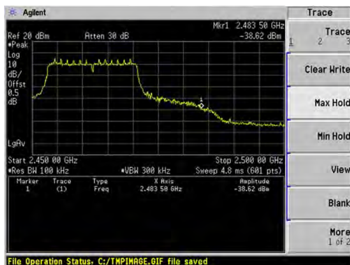
802.11n-20 MHz HIGH CHANNEL, Reference level
