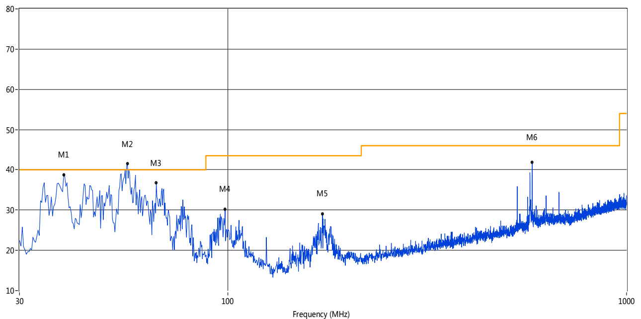
RE Test case_FCC 15C 30MHz-1GHz
