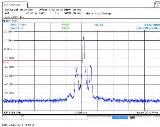
Band 2 QPSK 1.4 MHz RB1#0 LCH
