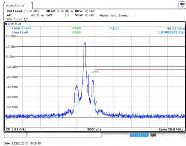
Band 2 QPSK 1.4 MHz RB1#0 HCH
