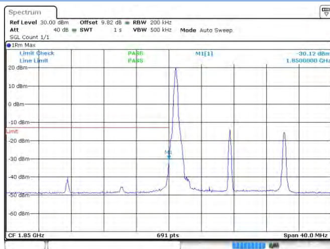
Band 2 16-QAM 15 MHz RB1#0 LCH
