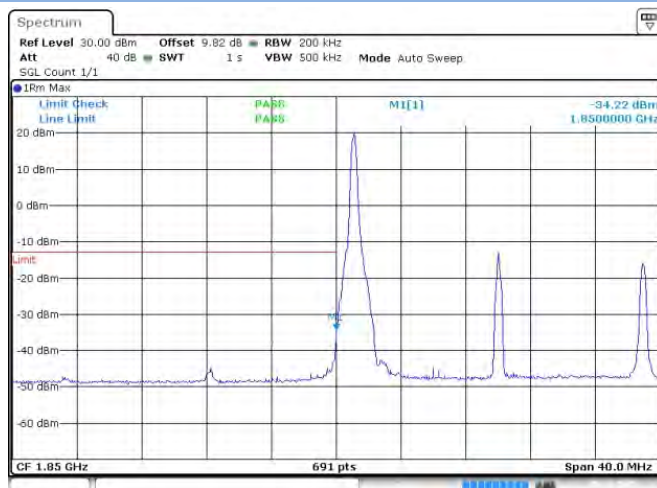
Band 2 16-QAM 20 MHz RB1#0 LCH
