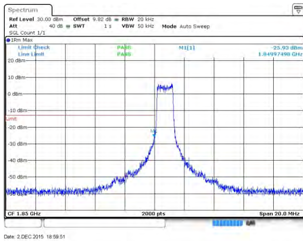
Band 2 QPSK 1.4 MHz RB1#6 LCH
