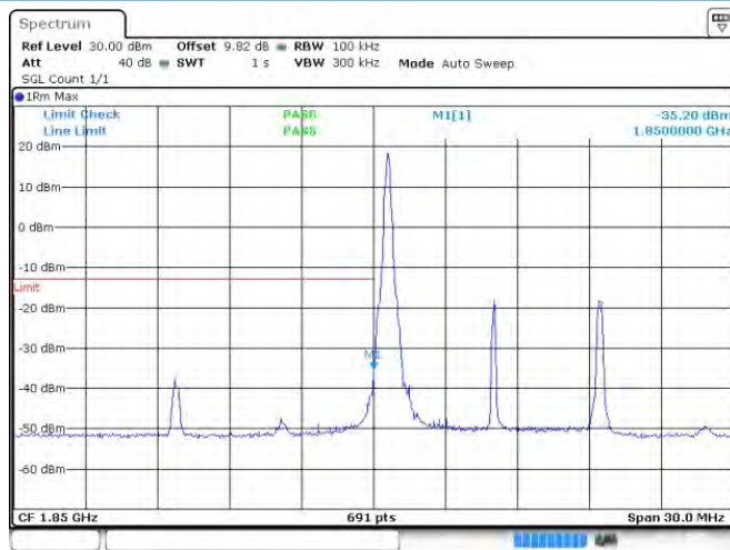
Band 2 16-QAM 10 MHz RB1#0 LCH
