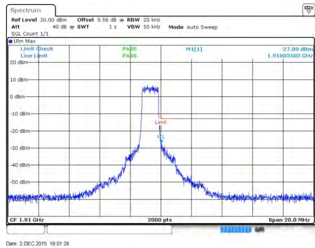
Band 2 QPSK 1.4 MHz RB1#6 HCH
