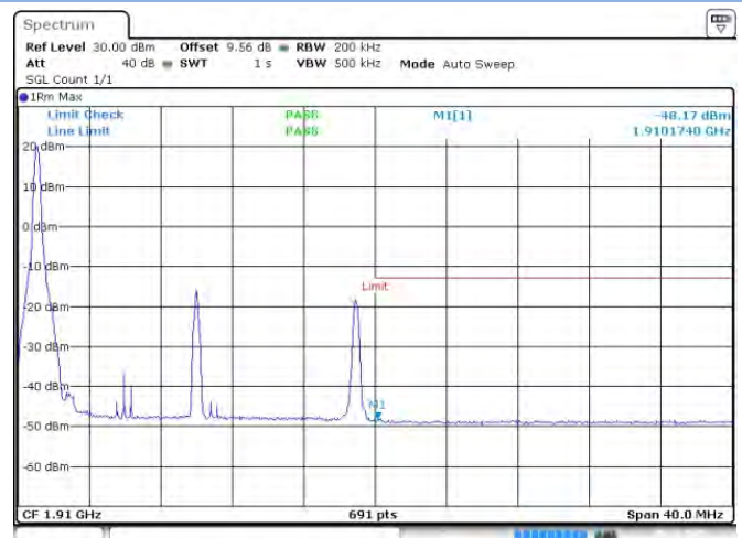
Band 2 16-QAM 20 MHz RB1#0 HCH
