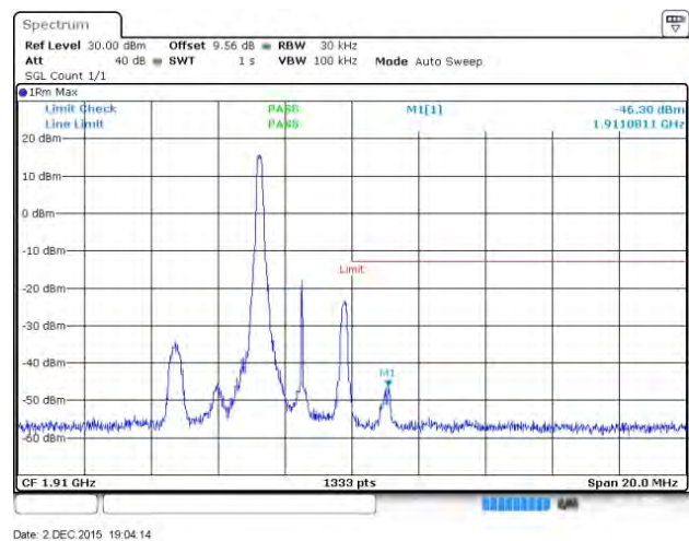
Band 2 QPSK 3 MHz RB1#0 HCH
