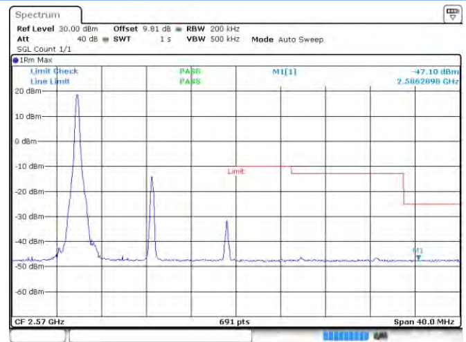
Band 7 16-QAM 15 MHz RB1#0 HCH
