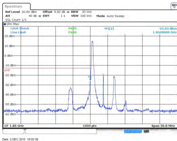
Band 2 QPSK 3 MHz RB1#0 LCH
