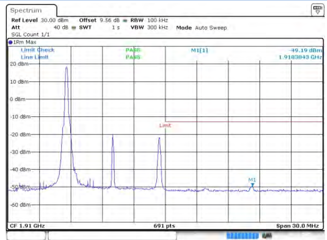
Band 2 16-QAM 10 MHz RB1#0 HCH
