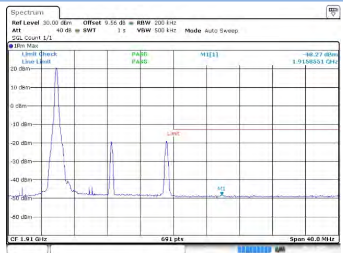
Band 2 16-QAM 15 MHz RB1#0 HCH
