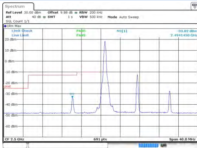
Band 7 16-QAM 15 MHz RB1#0 LCH
