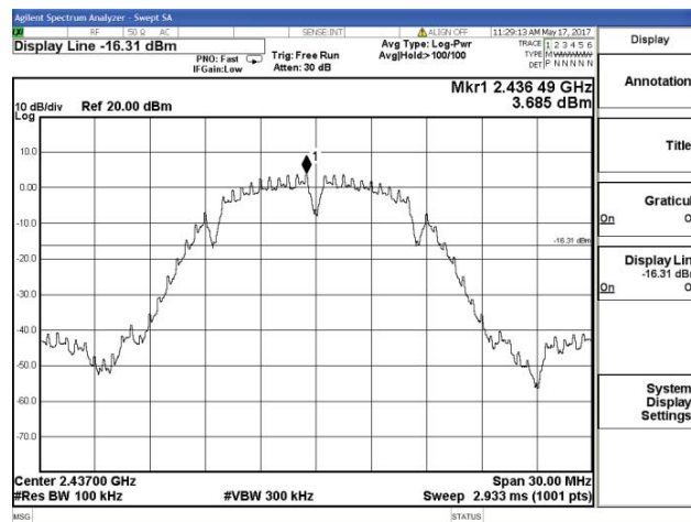
802.11b_Middle Channel
