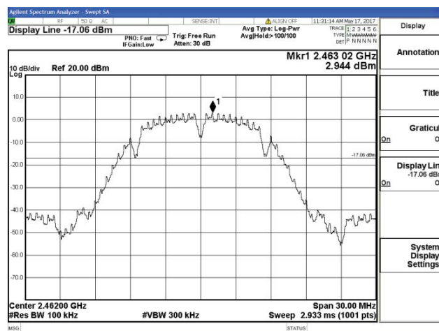
802.11b_High Channel
