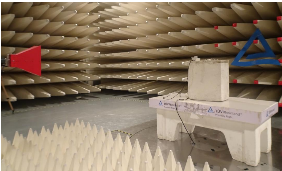
Photo 10: Horn antenna with horizontal polarization
