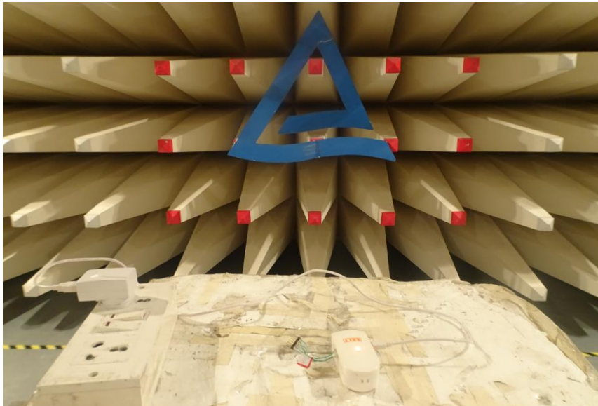
Photo 13: EUT setup
