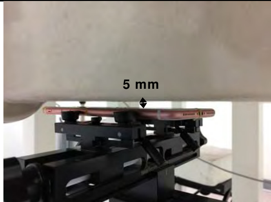
Fig.7 EUT Front side to flat phantom (No Case)
