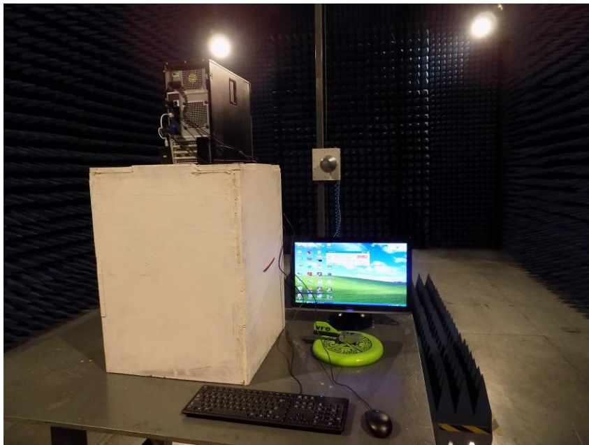
Above 1GHz
