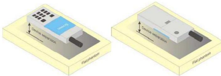
Picture D.1 Test positions for body-worn devices
