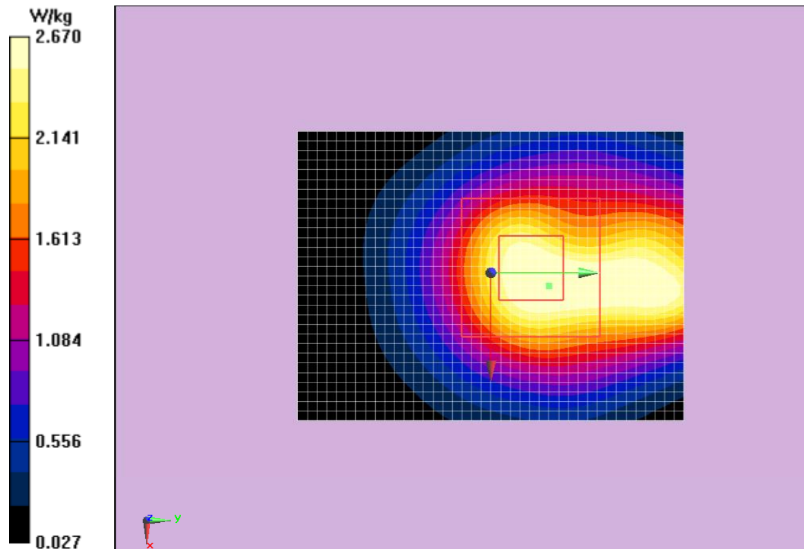
Fig.7 1900 MHz CH661
