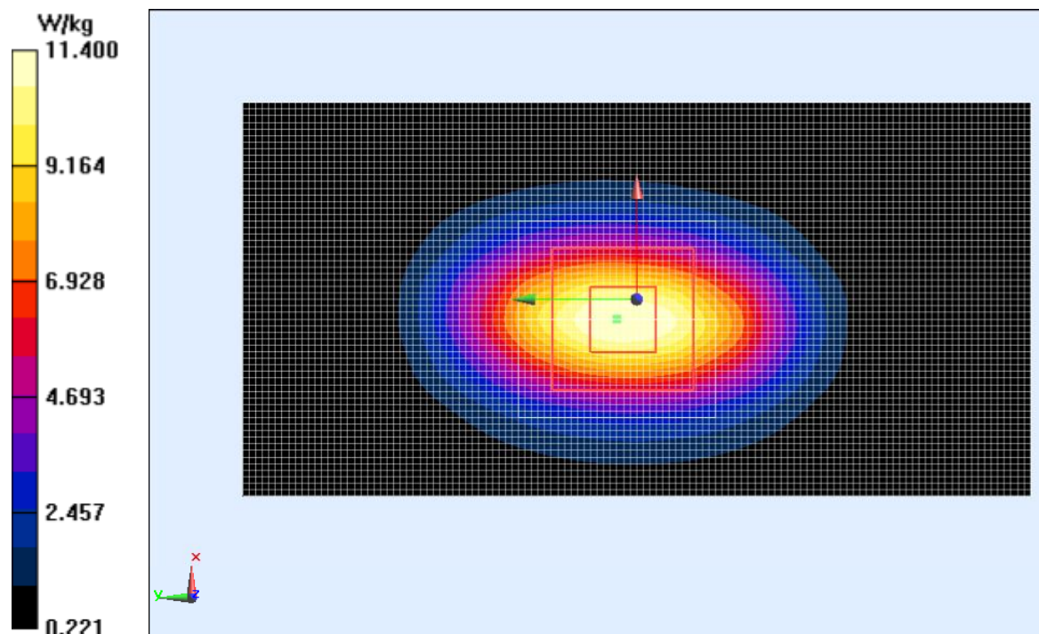
Fig.B.2 validation 835MHz 250mW
