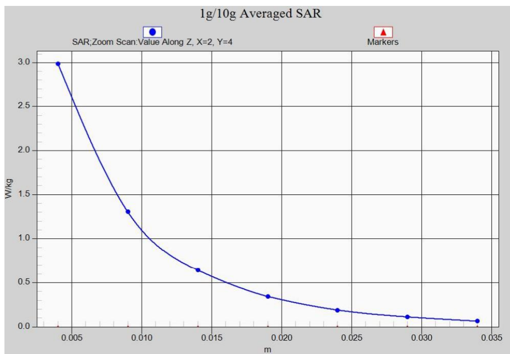
Fig.8-1 Z-Scan at power reference point (1900 MHz CH512)
