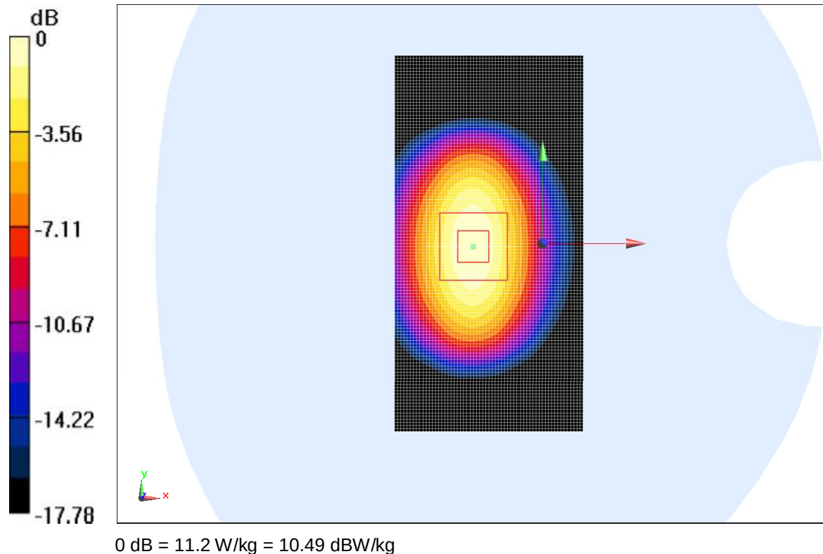
Fig.B.3 validation 1900MHz 250mW
