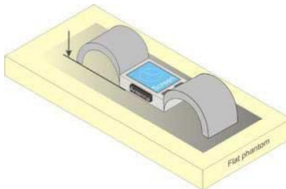
Picture D.2 Test position for limb-worn devices
