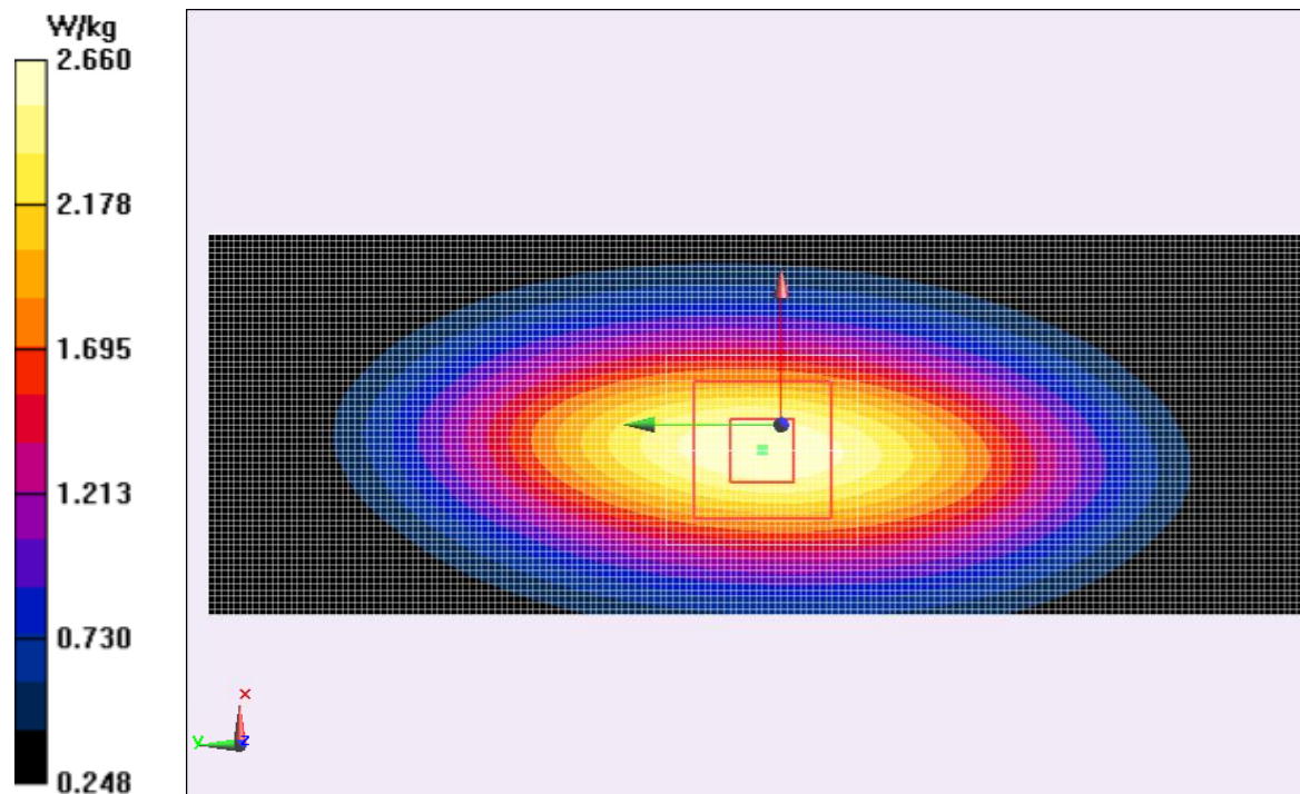
Fig.B.1 validation 835MHz 250mW
