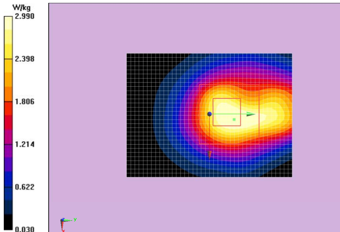
Fig.8 1900 MHz CH512
