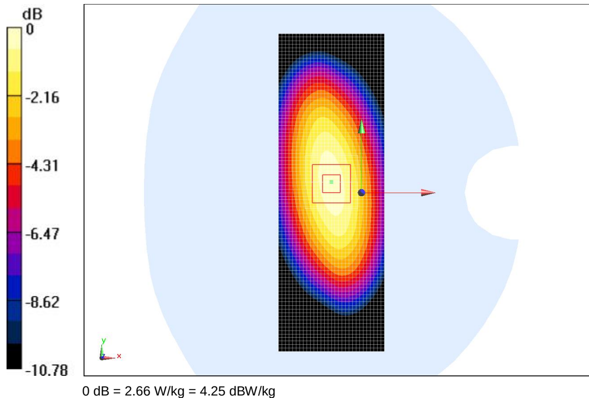
Fig.B.1 validation 835MHz 250mW
