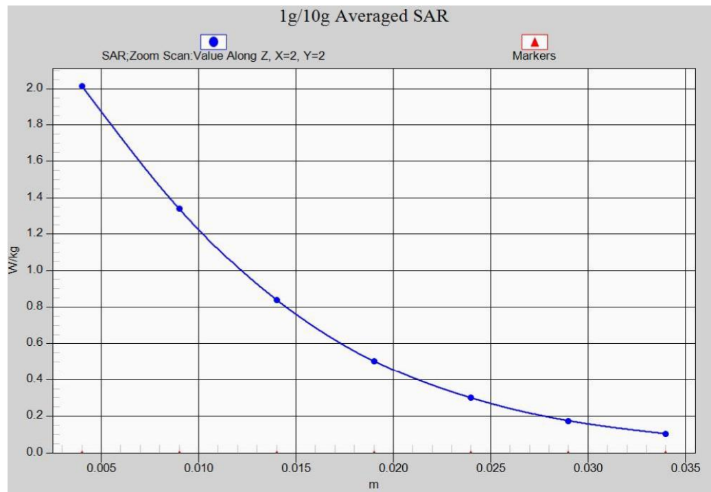
Fig.6-1 Z-Scan at power reference point (1900 MHz CH810)
