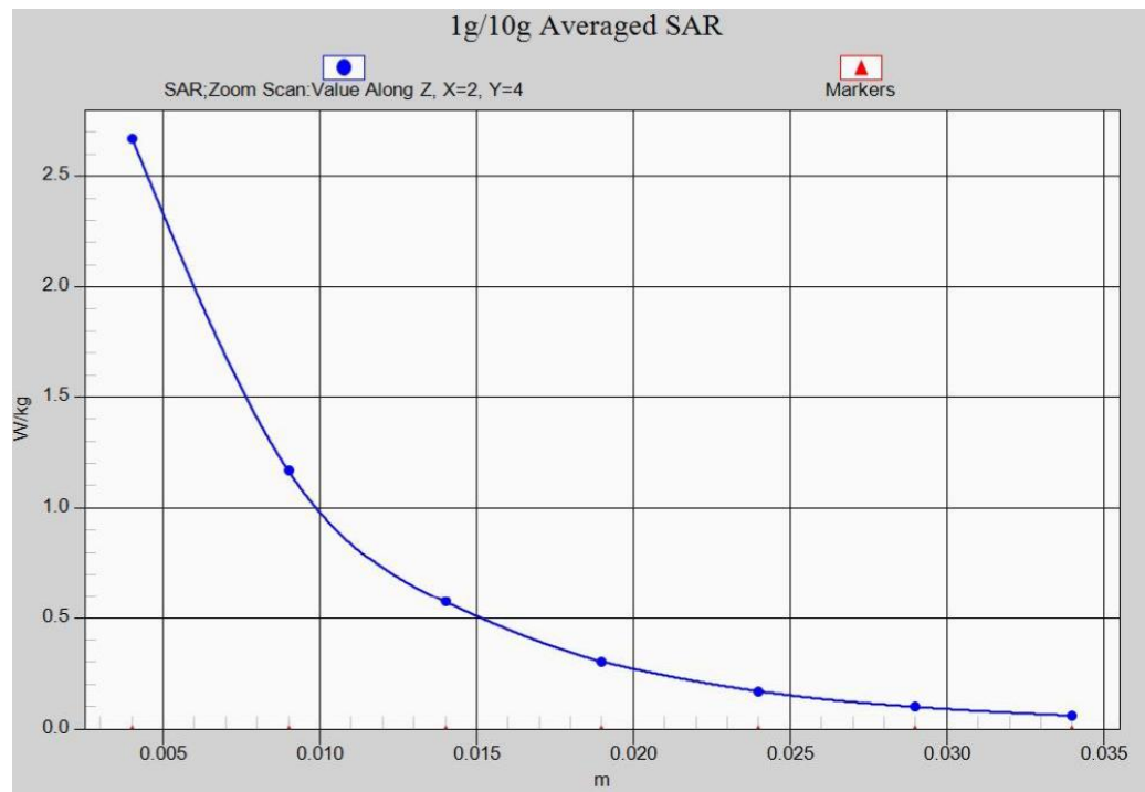
Fig.7-1 Z-Scan at power reference point (1900 MHz CH661)
