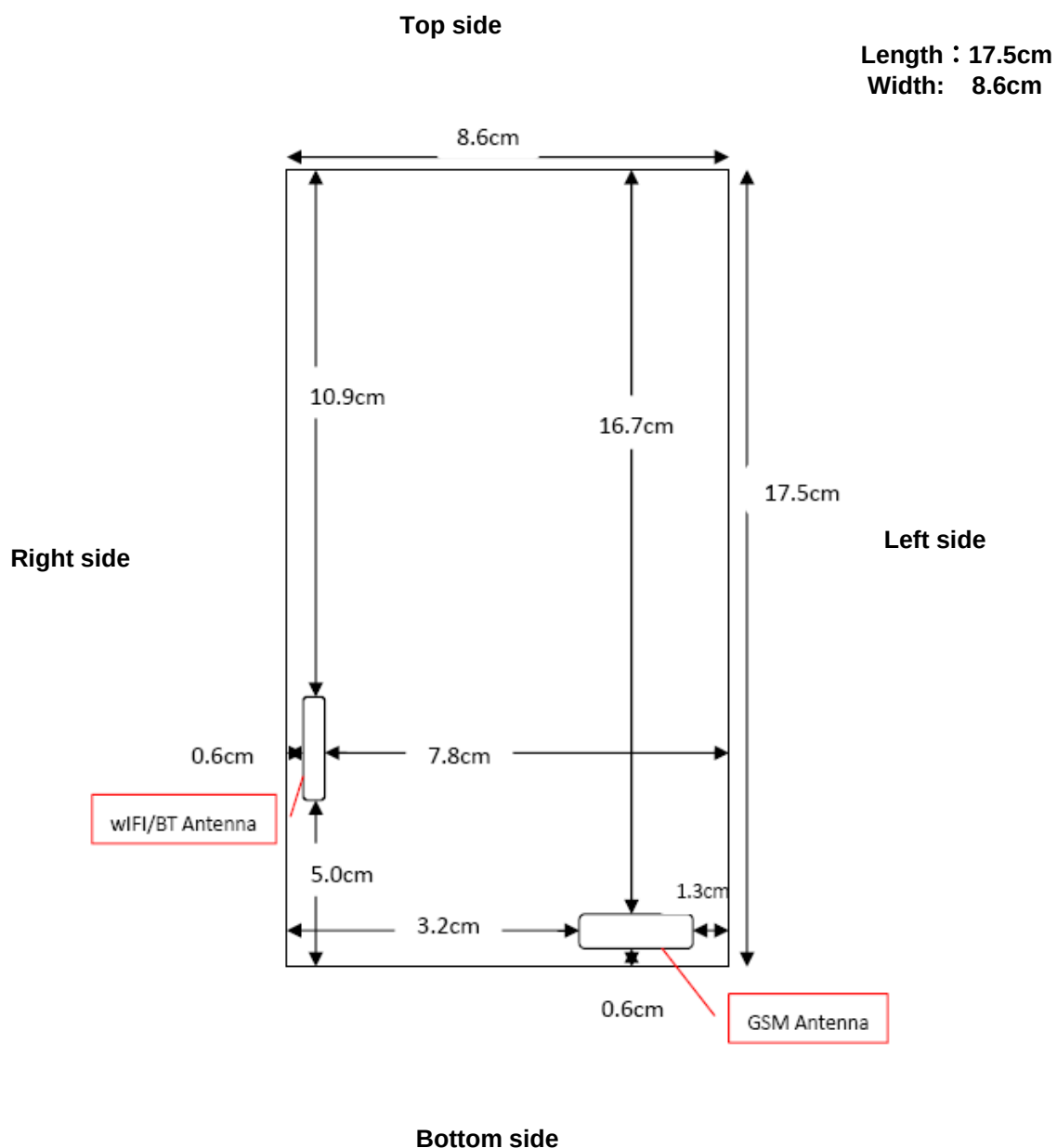
Figure1: The antenna position of the DUT
