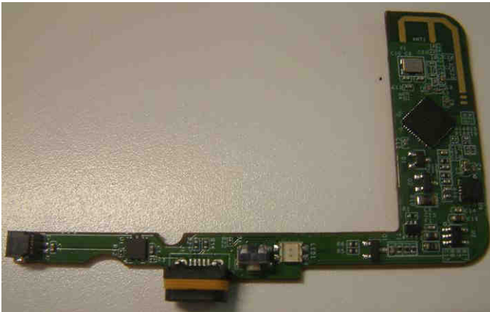
Cover removed
