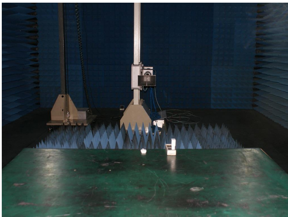
Photograph 2: Set-up for Radiated emissions, UpRight Battery Charging with AC/DC adapter, above 1 GHz
