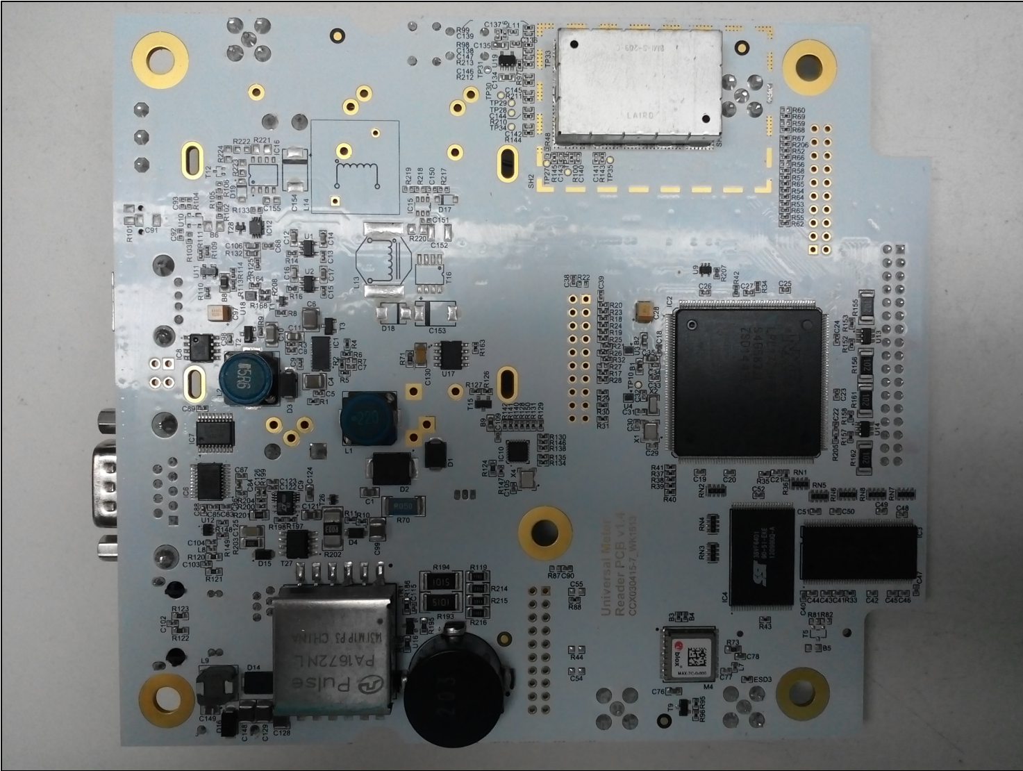
Figure 4: PCB Bottom with Shield
