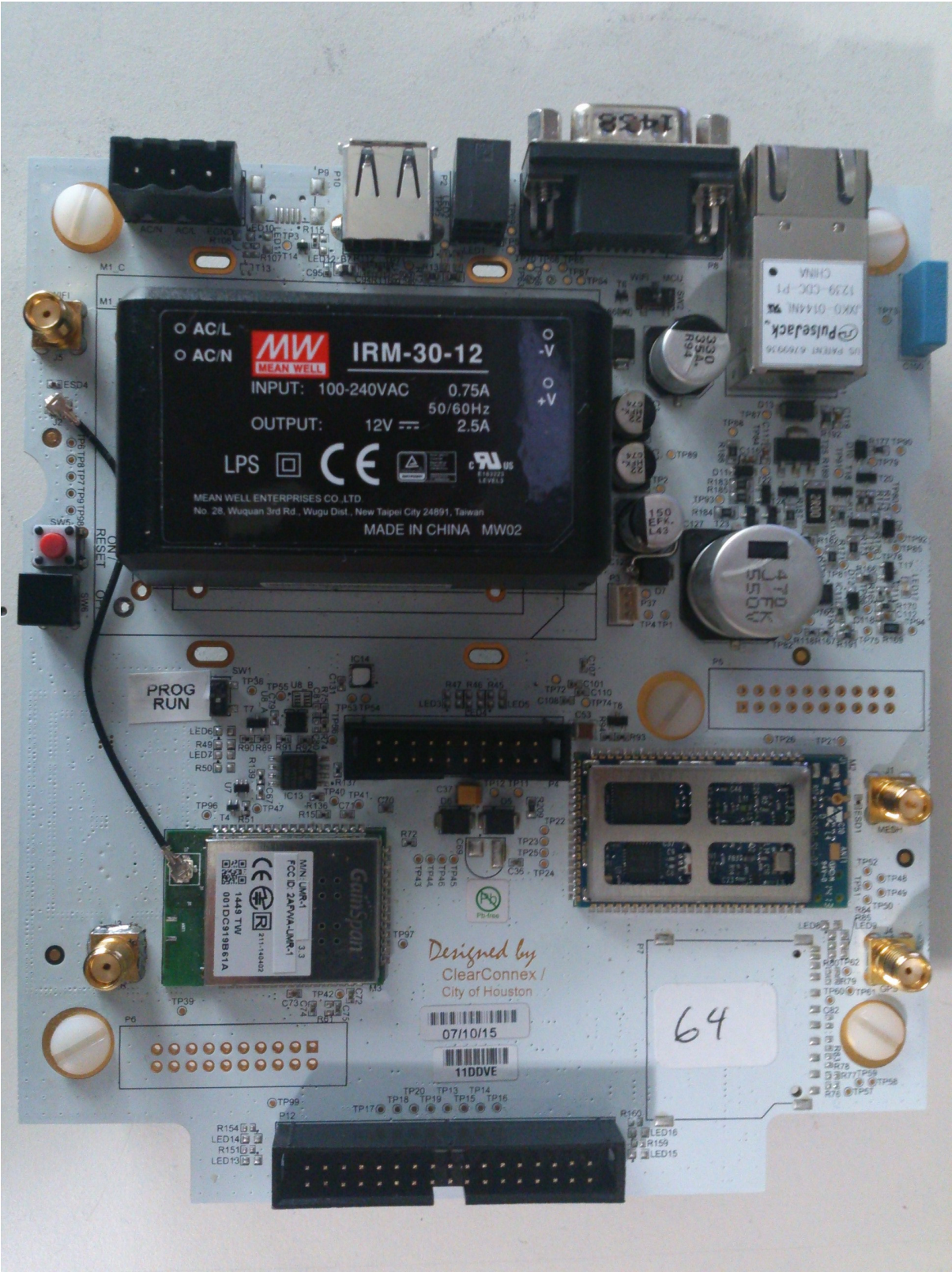
Figure 3: PCB Top without Shield
