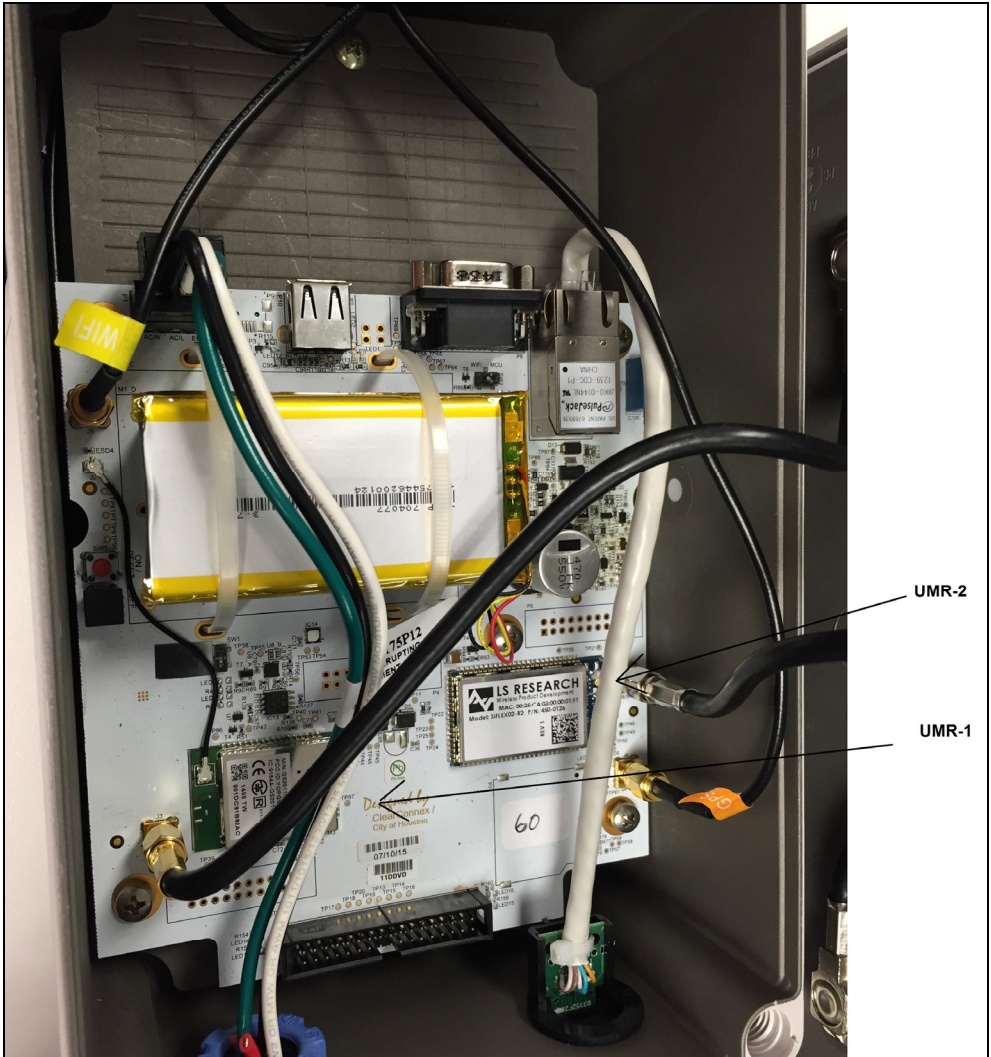
Figure 1: Inside View
