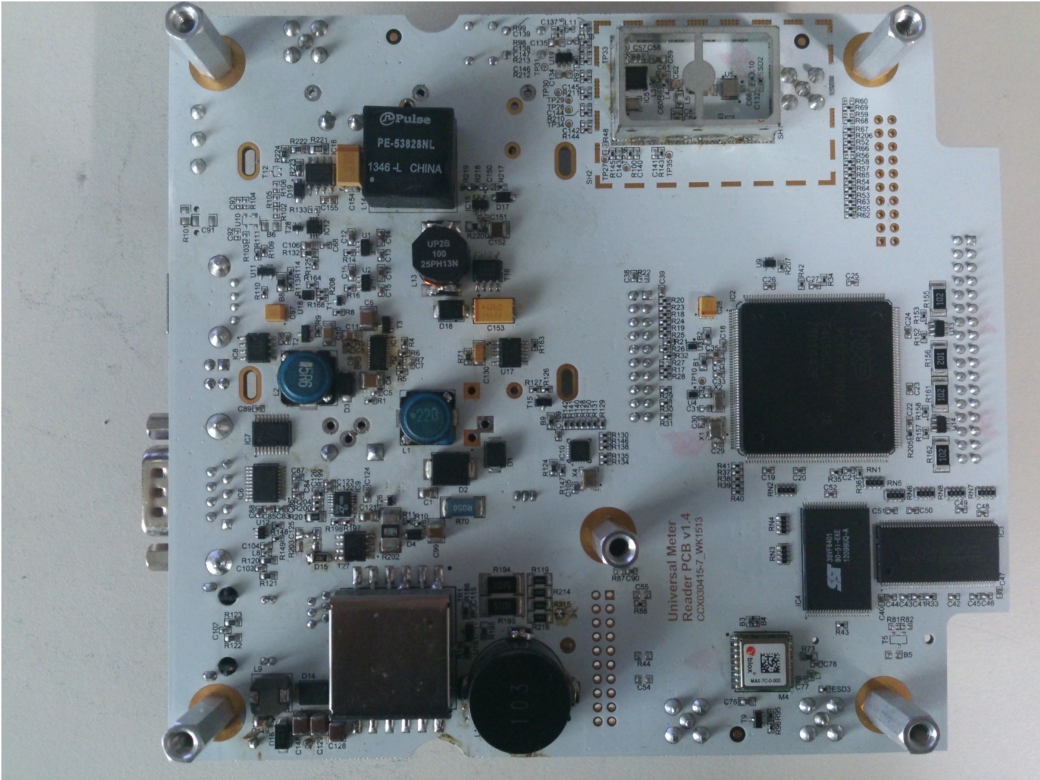
Figure 5: PCB Bottom without Shield
