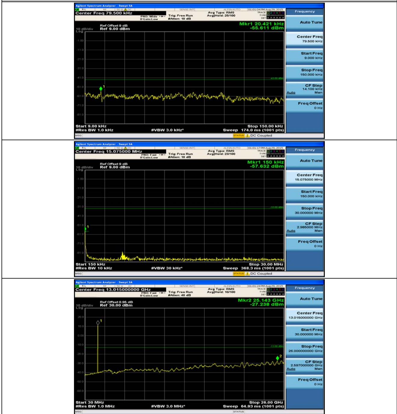
(Channel Bandwidth: 1.4 MHz)_MCH_16QAM_1RB#5
