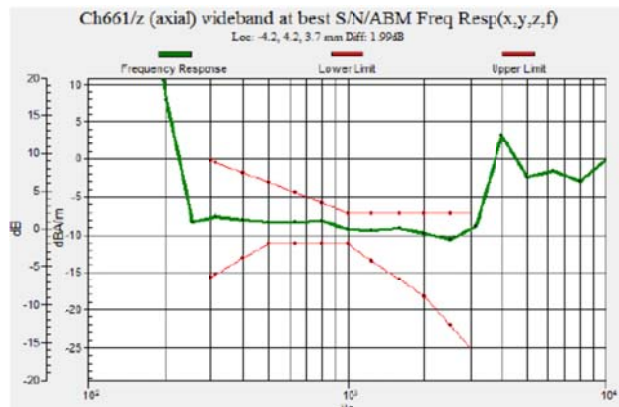
Fig 7.2 GSM1900 Ch661
