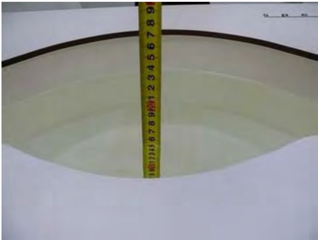
Picture 16: Liquid depth in the flat Phantom (5300 MHz, 15.3cm depth)
