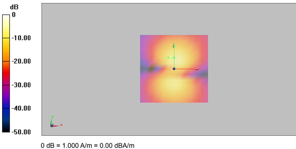
Figure 15 T-Coil WCDMA Band II Y transversal
