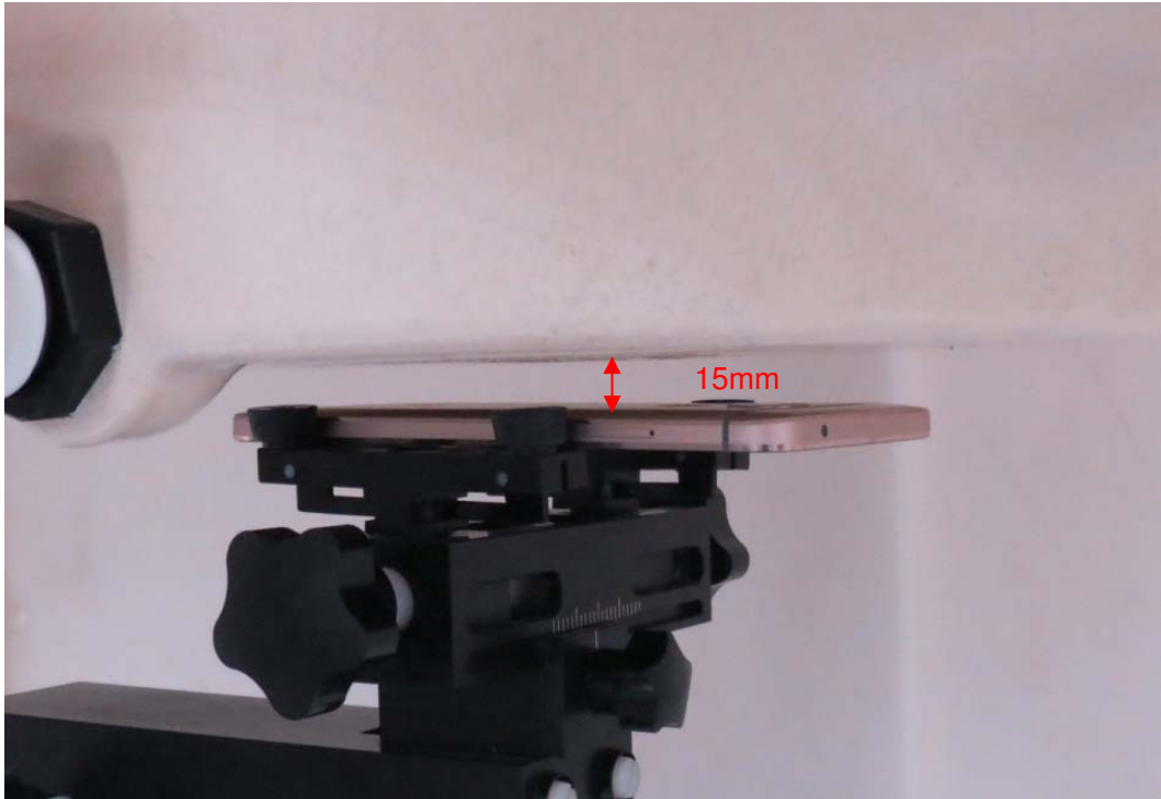
Picture 8: Back Side, the distance from handset to the bottom of the Phantom is 15mm
