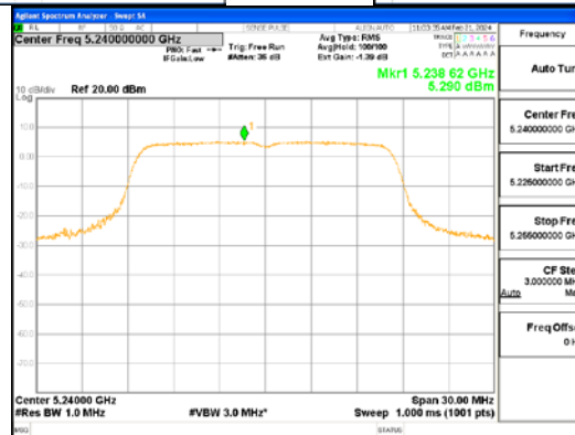
802.11a_UNII 1
