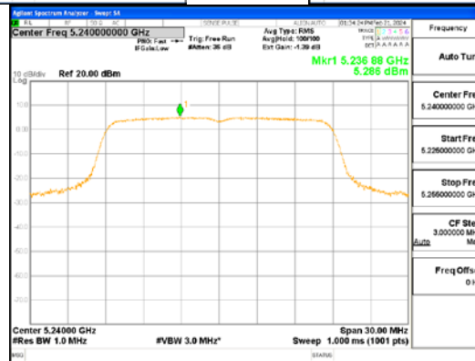
802.11n_HT20_UNII 1
