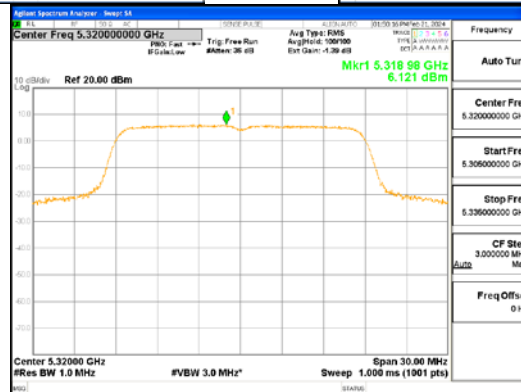
802.11n_HT20_UNII 2A
