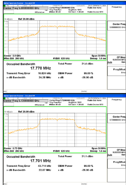
802.11n_HT20_UNII 2C
