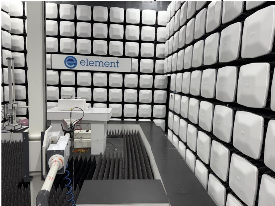
Radiated measurement(1 GHz ~10 GHz)
