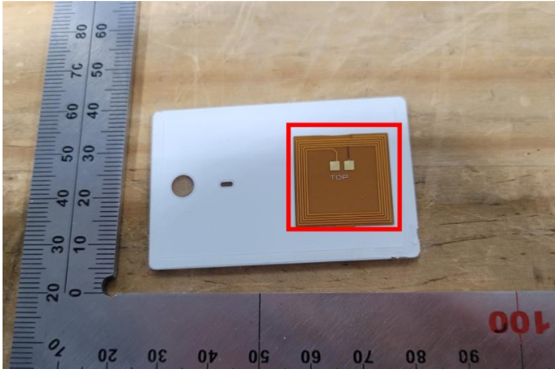
[NFC(Only Rx) Antenna]
