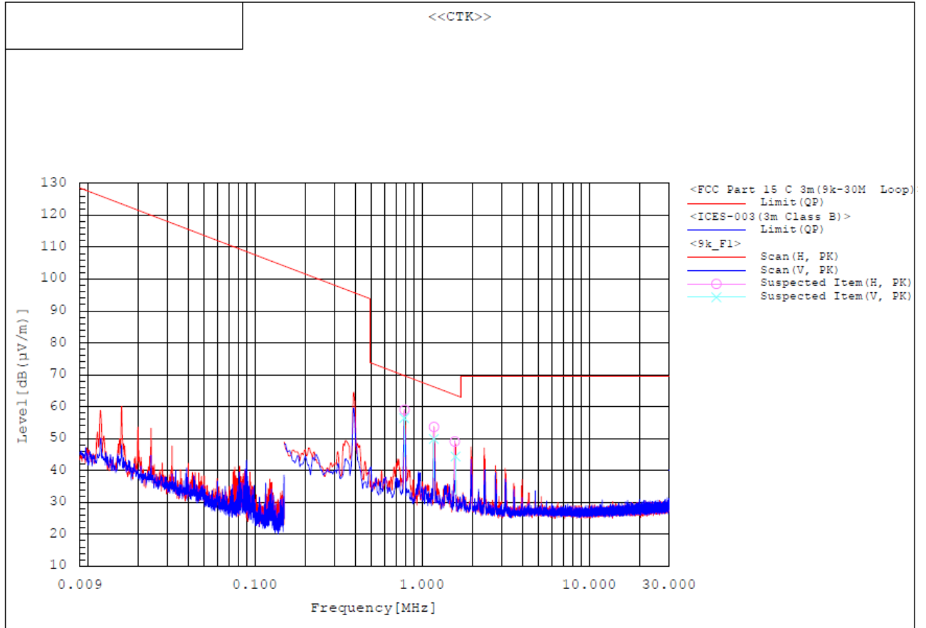
Spectrum Selection
