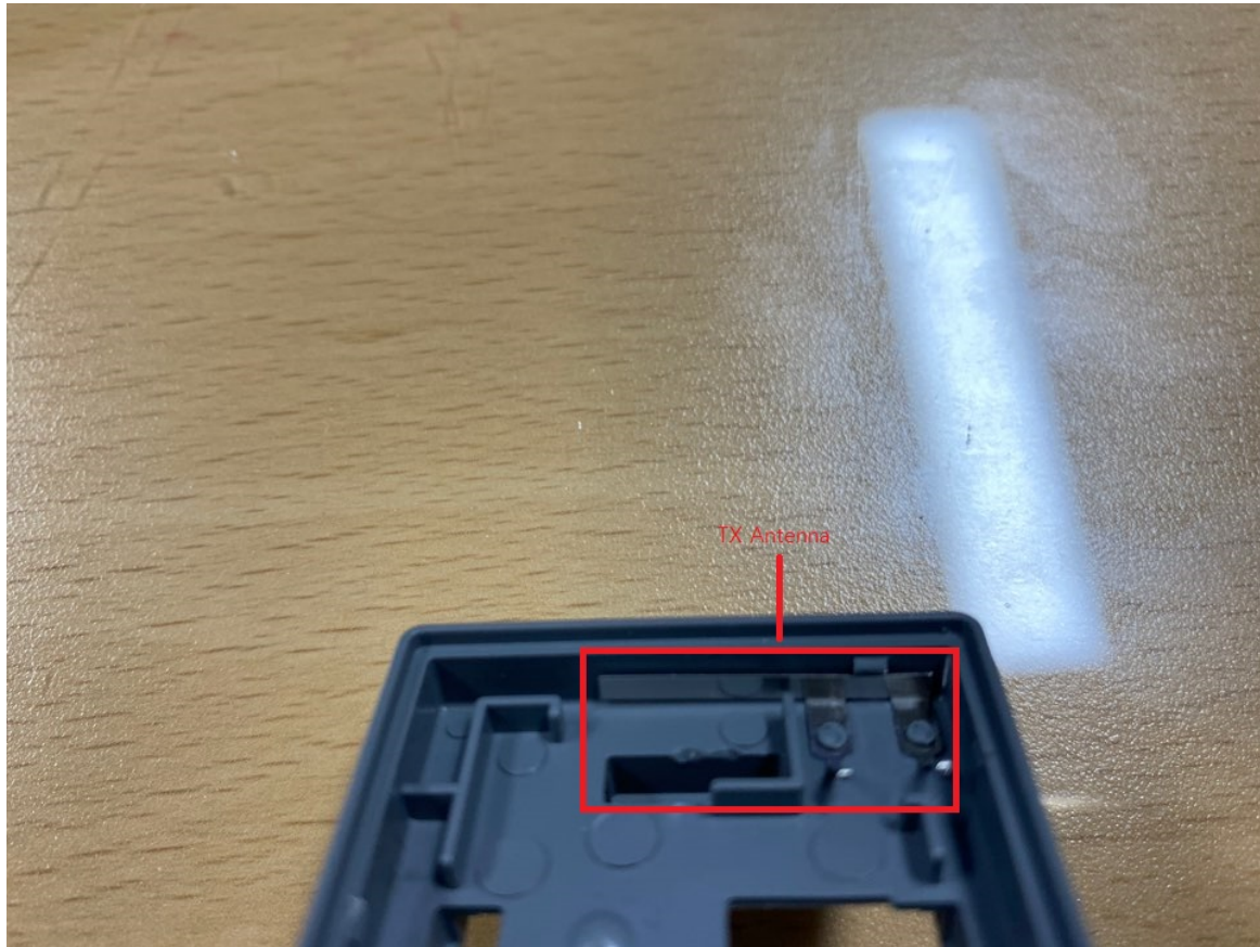
TX, RX Antenna
