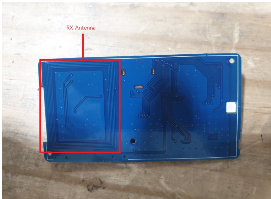
RX Antenna
