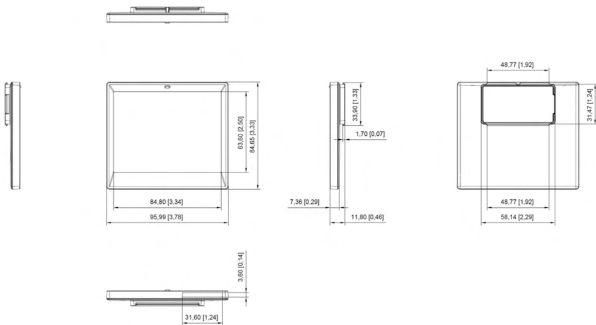
Figure 8. 4.2" MECHANICAL DIMENSION
