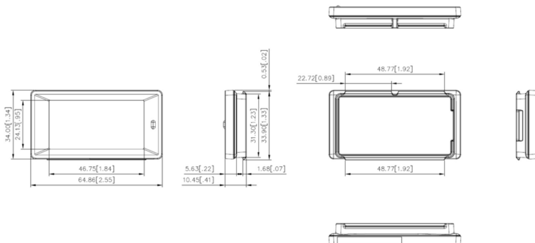
Figure 4. 2.1" MECHANICAL DIMENSION
