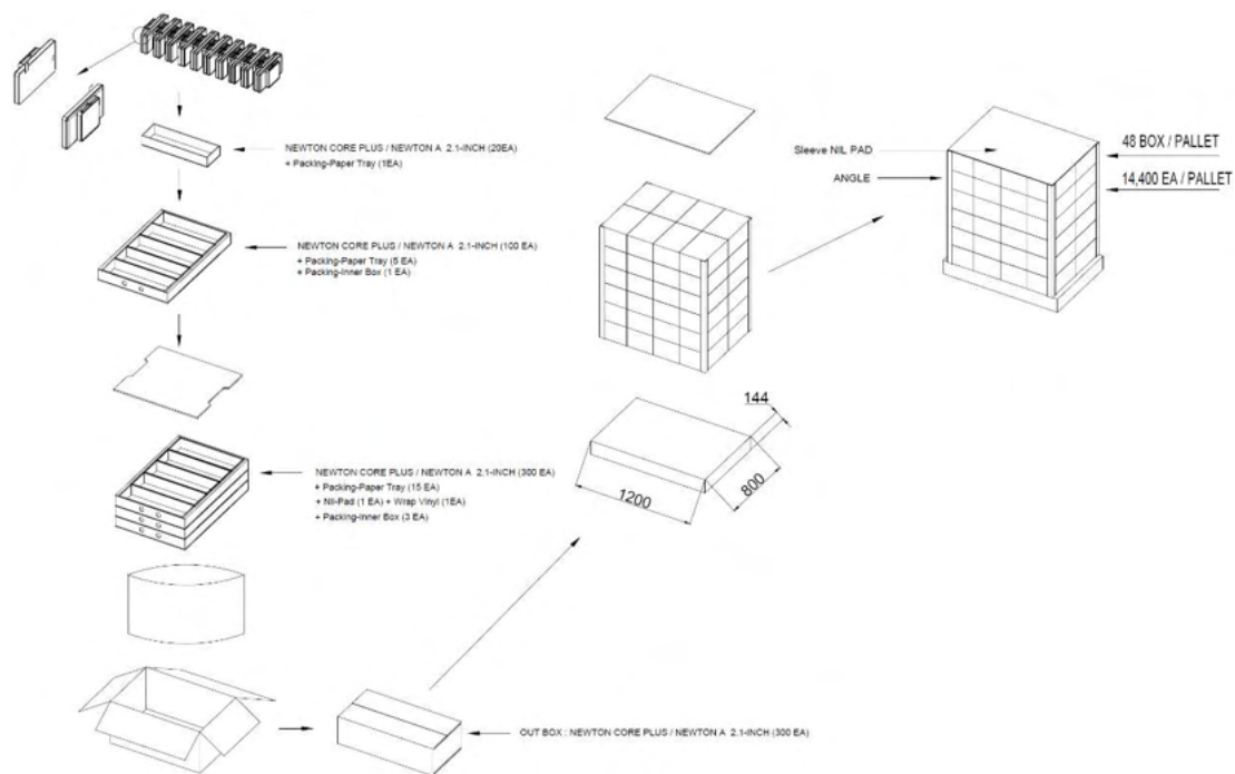
Figure 16. 2.1" PACKING-DIAGRAM (1,200 X 800)
