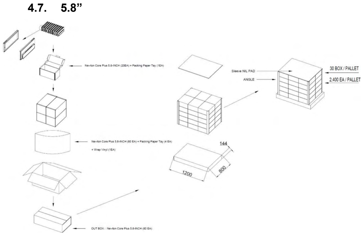
Figure 26. 5.8" PACKING-DIAGRAM (1,200 X 800)
