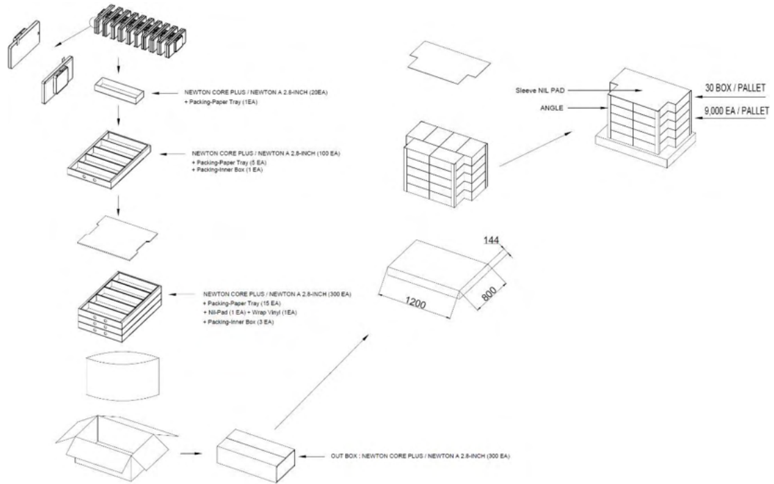
Figure 20. 2.8" PACKING-DIAGRAM (1,200 X 800)
