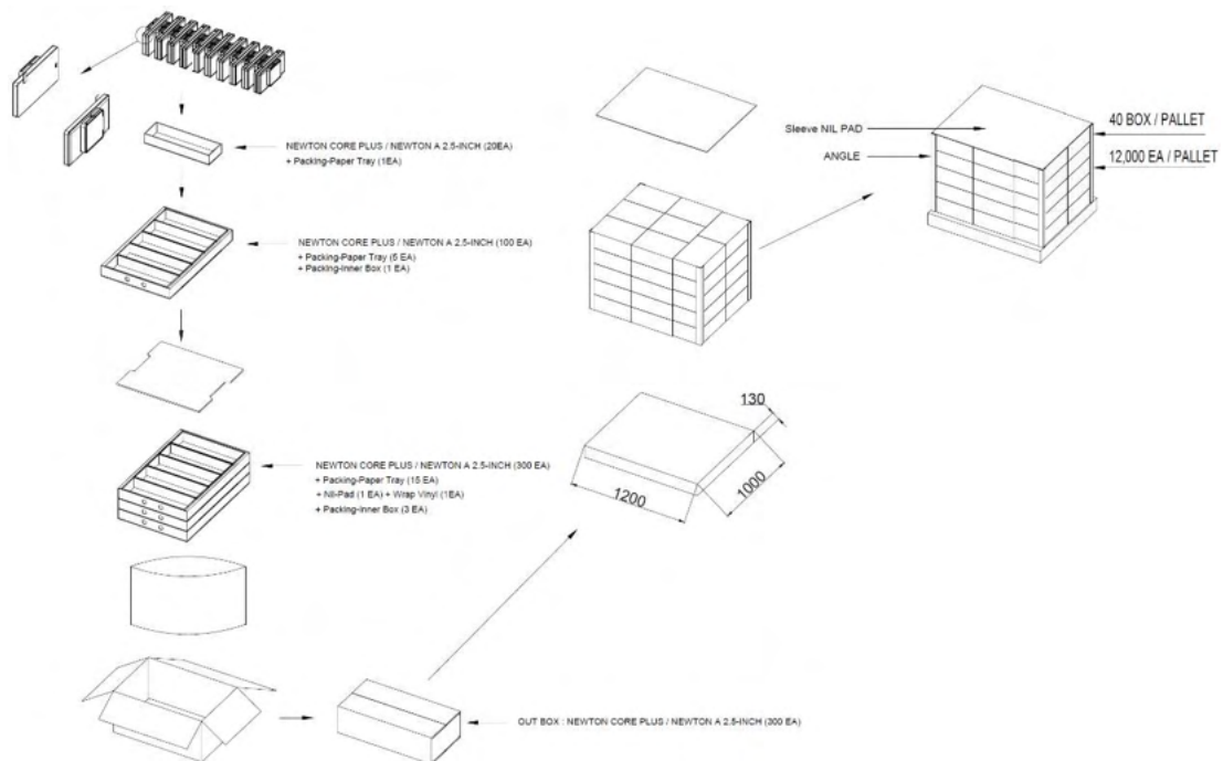
Figure 19. 2.5" PACKING-DIAGRAM (1,200 X 1,000)
