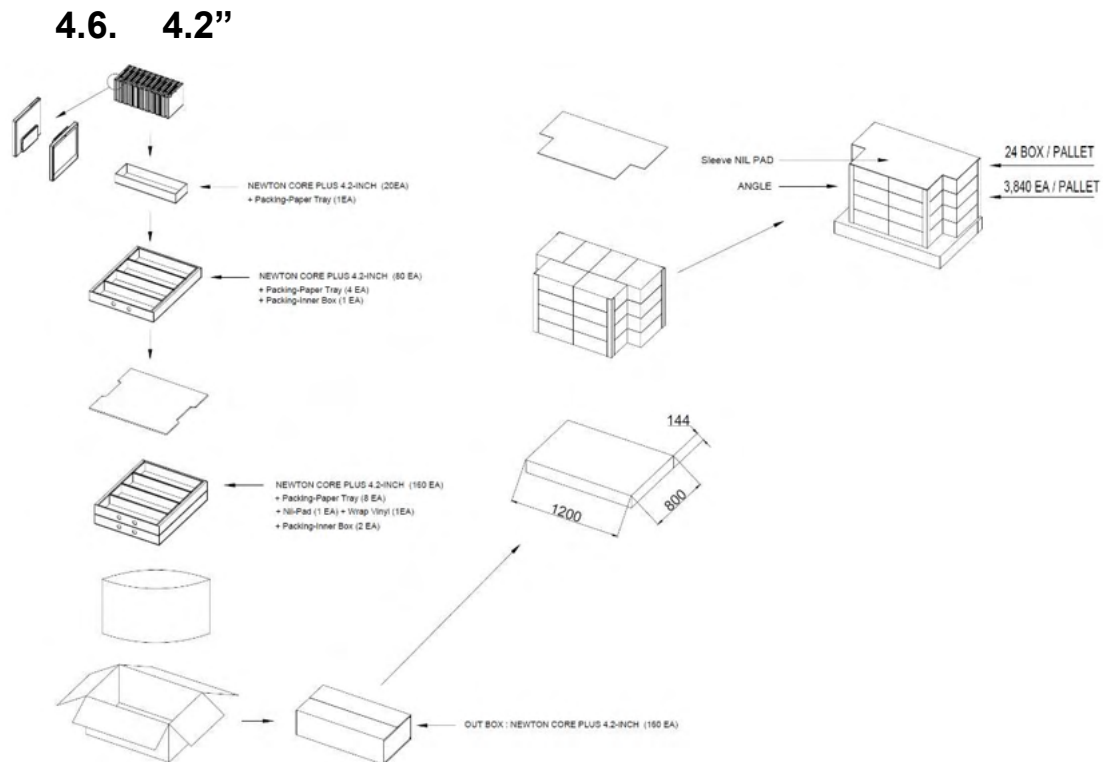
Figure 24. 4.2" PACKING-DIAGRAM (1,200 X 800)
