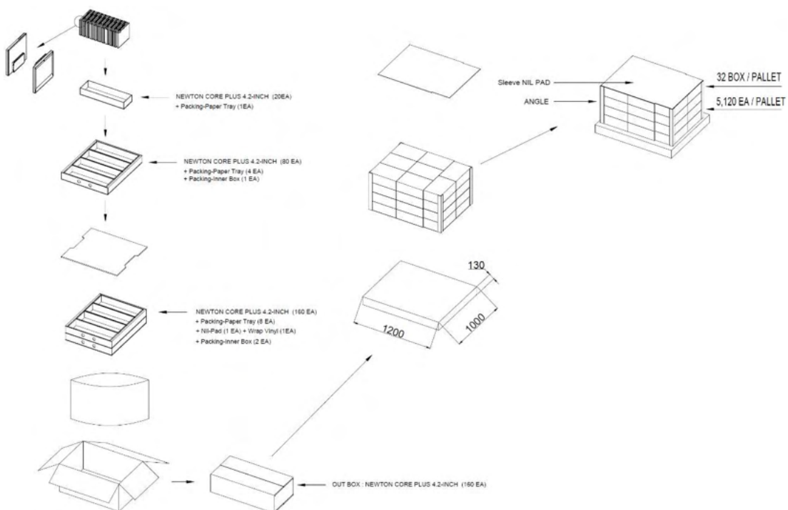
Figure 25. 4.2" PACKING-DIAGRAM (1,200 X 1,000)
