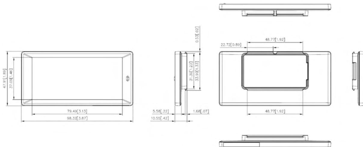
Figure 7. 3.5" MECHANICAL DIMENSION
