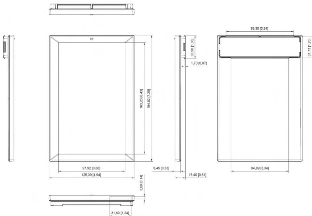
Figure 10. 7.5" MECHANICAL DIMENSION
