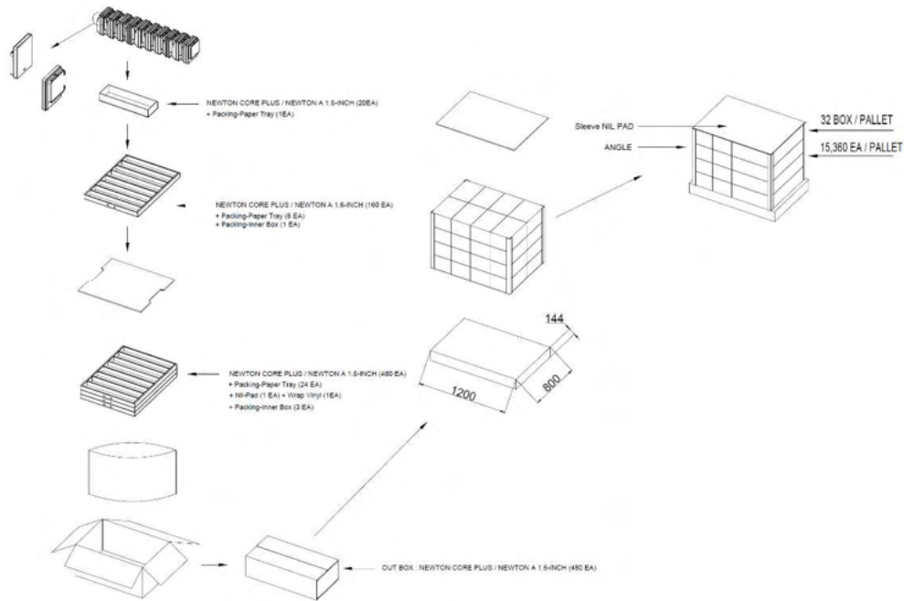
Figure 14. 1.6" PACKING-DIAGRAM (1,200 X 800)
