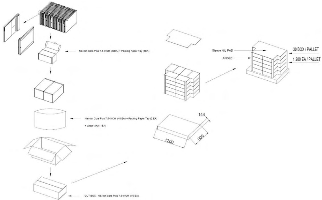
Figure 28. 7.5" PACKING-DIAGRAM (1,200 X 800)
