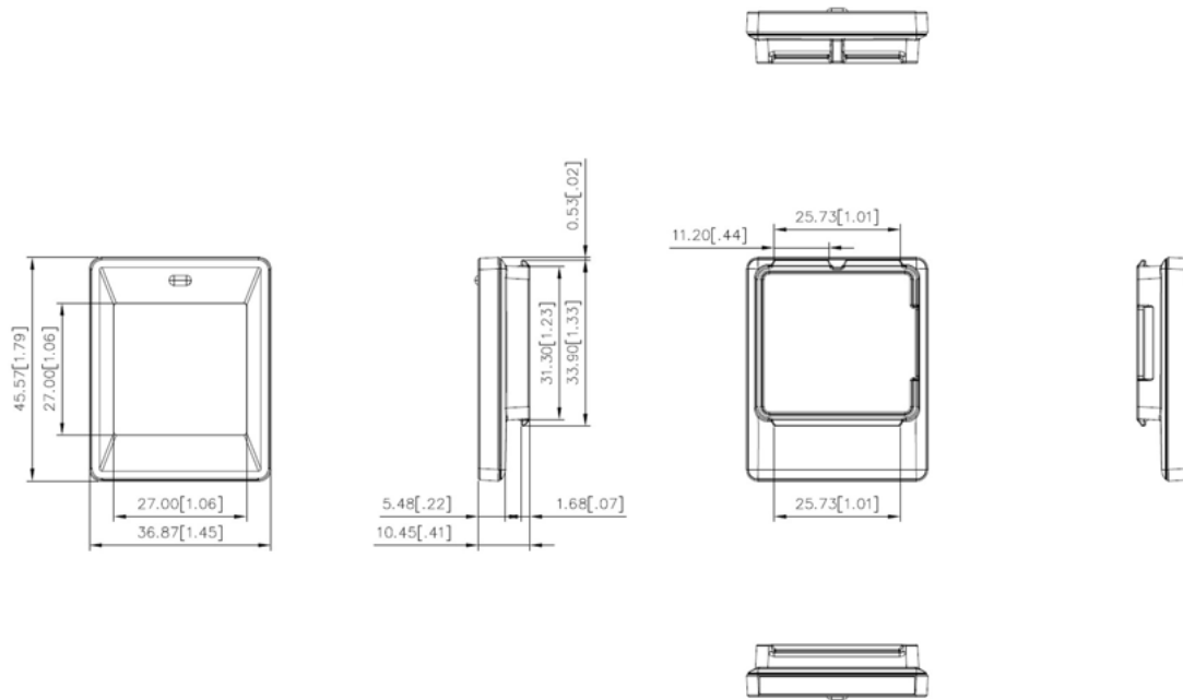
Figure 3. 1.6" MECHANICAL DIMENSION
