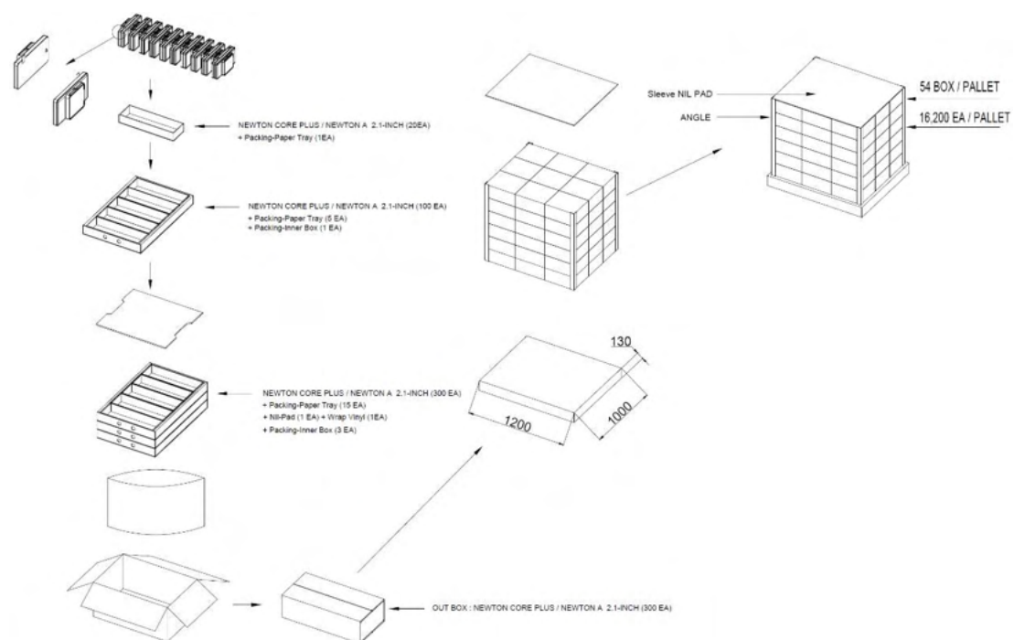
Figure 17. 2.1" PACKING-DIAGRAM (1,200 X 1,000)
