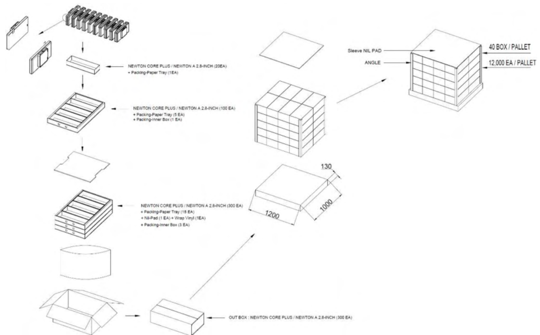
Figure 21. 2.8" PACKING-DIAGRAM (1,200 X 1,000)
