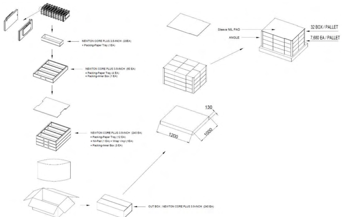
Figure 23. 3.5" PACKING-DIAGRAM (1,200 X 1,000)
