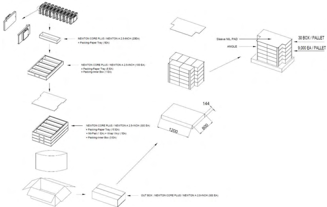
Figure 18. 2.5" PACKING-DIAGRAM (1,200 X 800)
