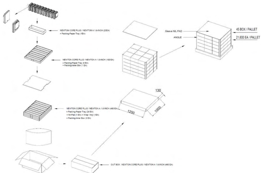
Figure 15. 1.6" PACKING-DIAGRAM (1,200 X 1,000)
