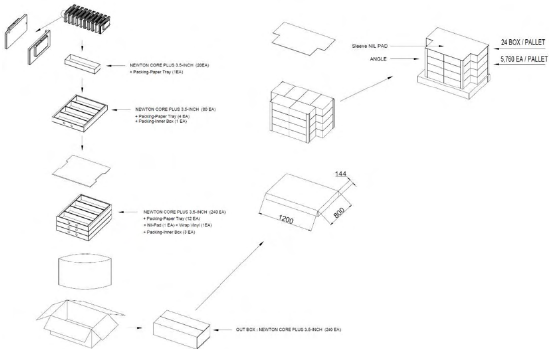
Figure 22. 3.5" PACKING-DIAGRAM (1,200 X 800)
