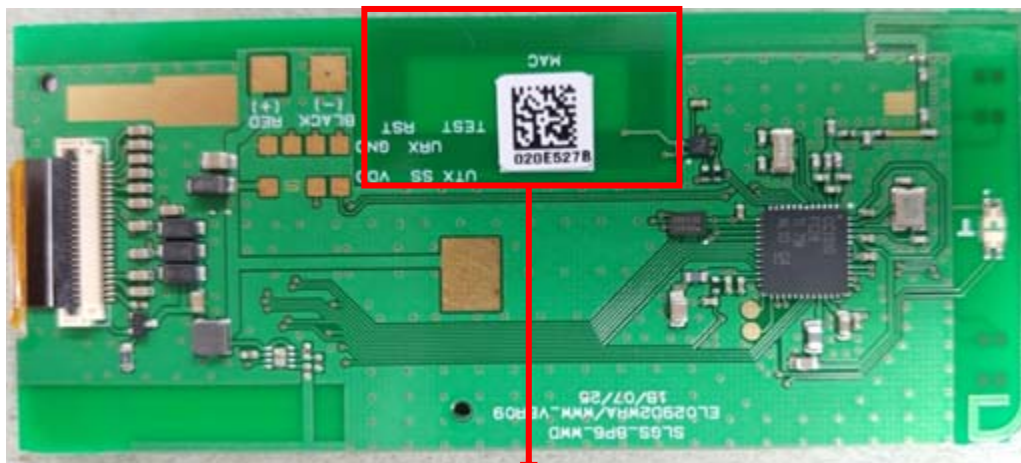
NFC receiving Antenna(RX)
