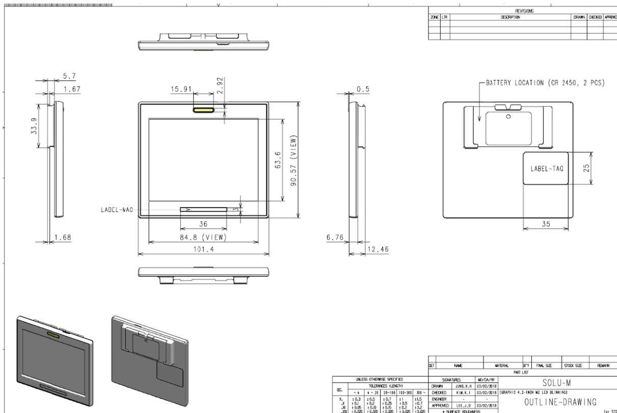
Figure 5. 2.9 Mechanical Dimension
