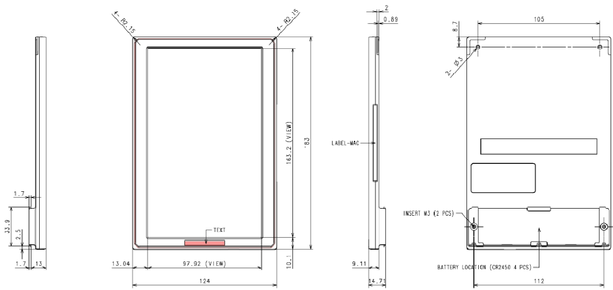
Figure 6.7.4”Mechanical Dimension
