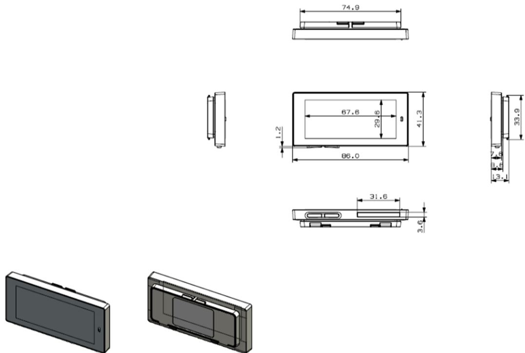
Figure 6. 2.9" Mechanical Dimension
