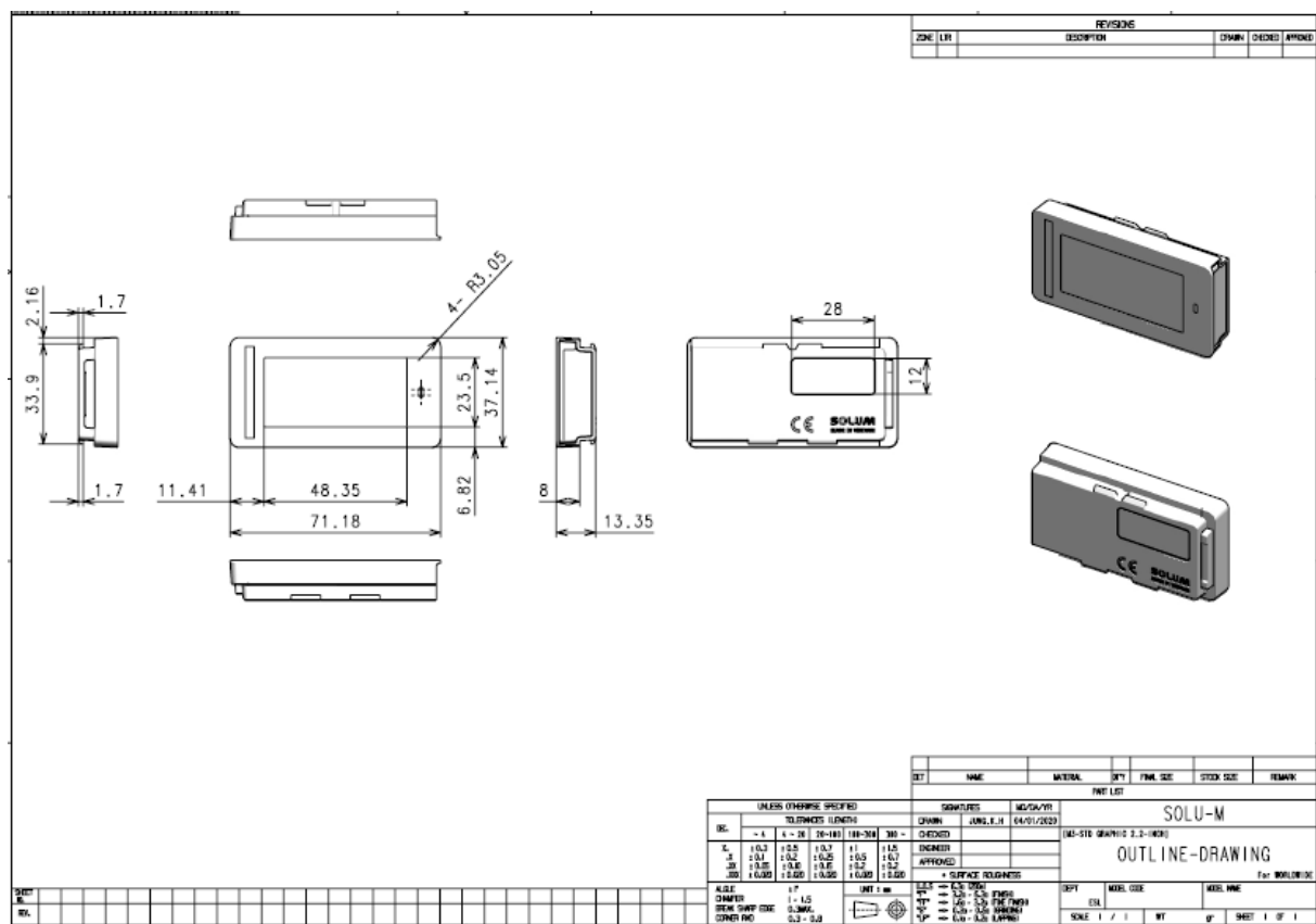
Figure 4.2.2" Mechanical Dimension
