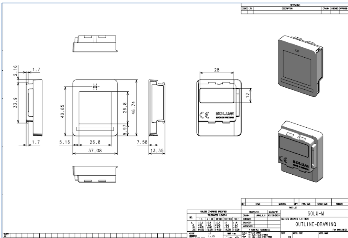
Figure 3. 1.6" Mechanical Dimension
