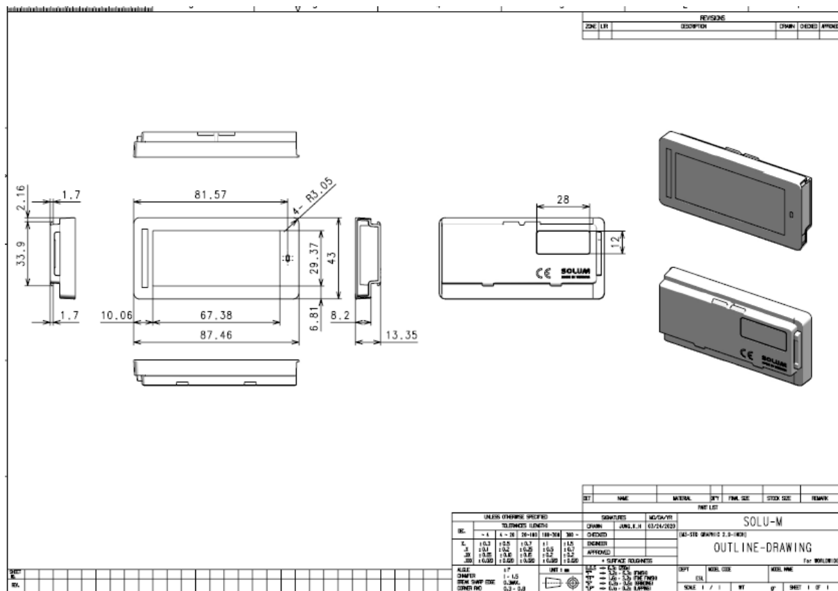
Figure 6. 2.9" Mechanical Dimension
