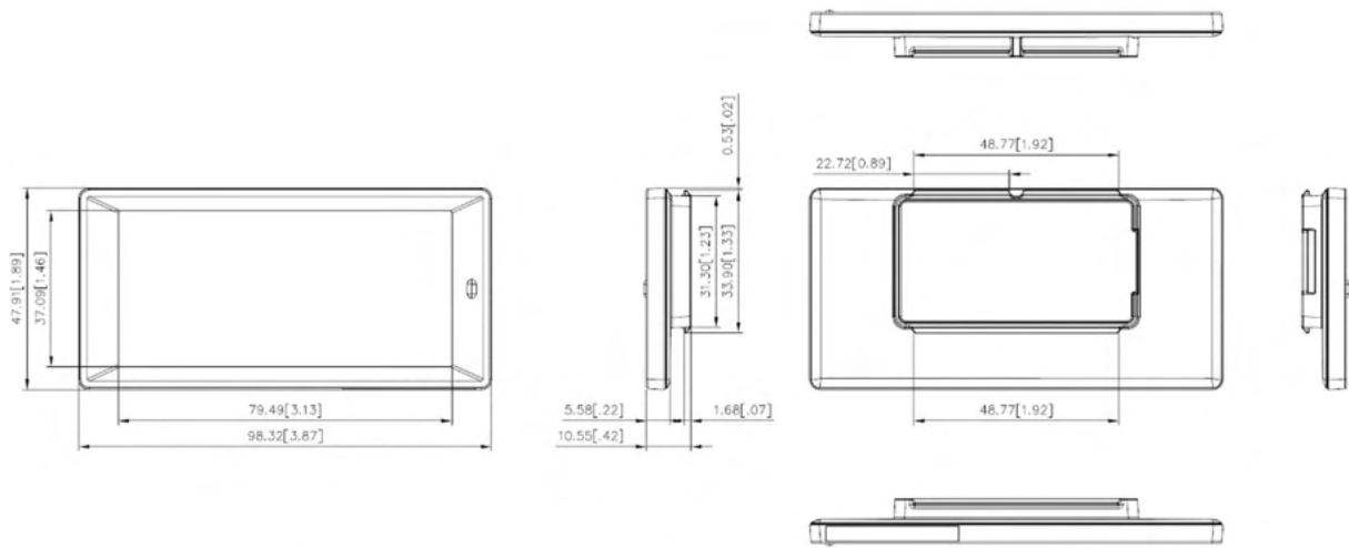
Figure 7. 3.5" MECHANICAL DIMENSION
