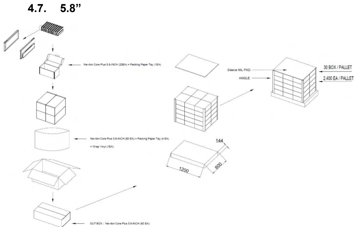
Figure 26. 5.8" PACKING-DIAGRAM (1,200 X 800)
