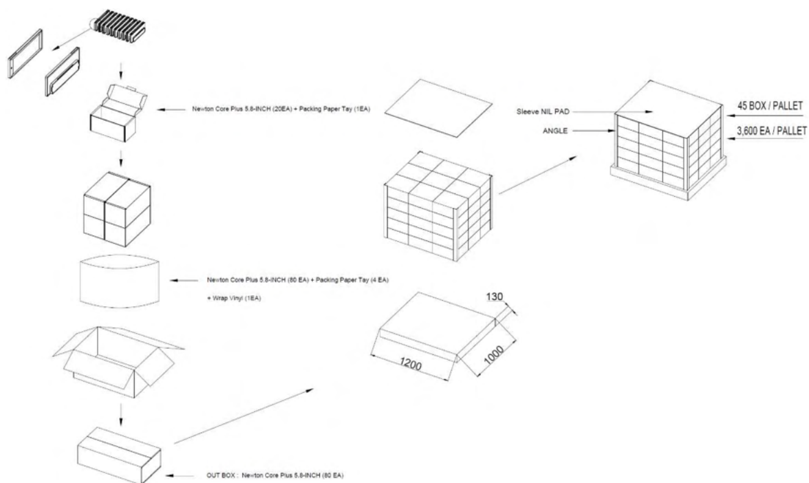
Figure 27. 5.8" PACKING-DIAGRAM (1,200 X 1,000)
