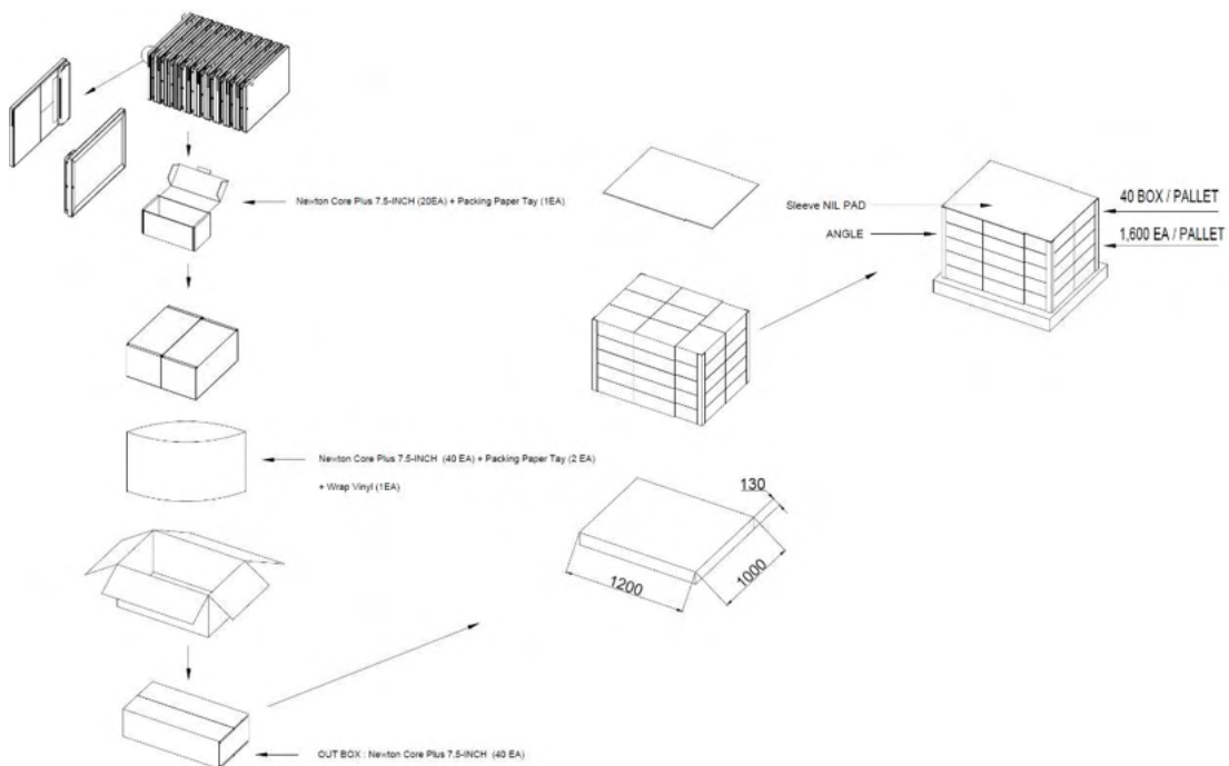
Figure 29. 7.5" PACKING-DIAGRAM (1,200 X 1,000)
