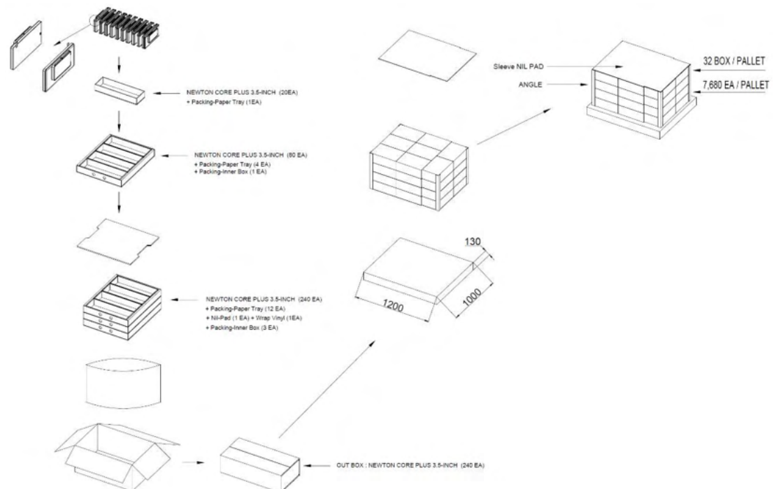
Figure 23. 3.5" PACKING-DIAGRAM (1,200 X 1,000)
