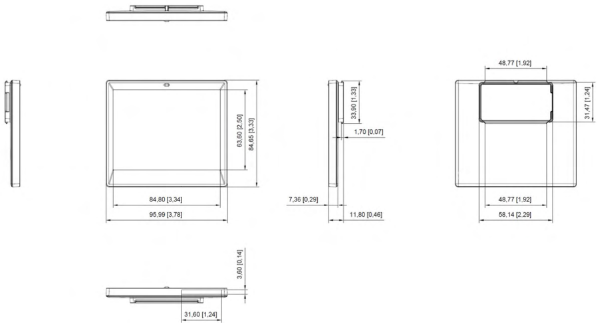
Figure 8. 4.2" MECHANICAL DIMENSION
