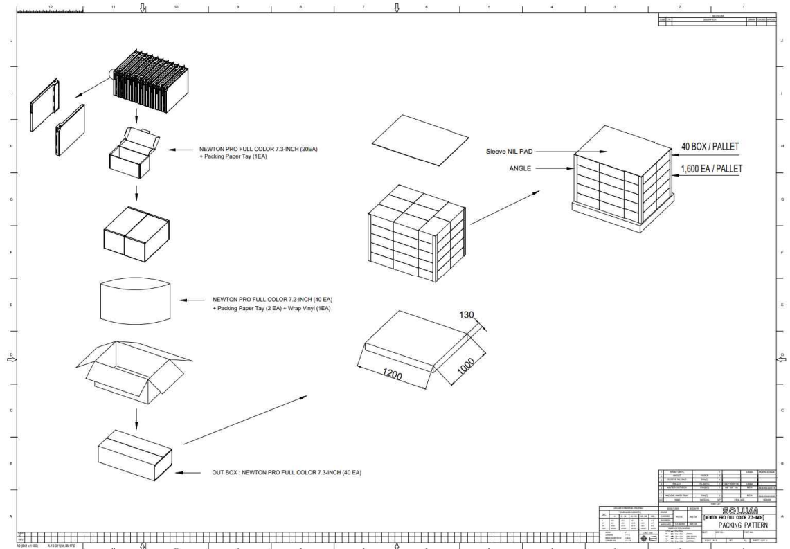
Figure 12. 7.3" Packing-Diagram (1,200 X 1,000)
