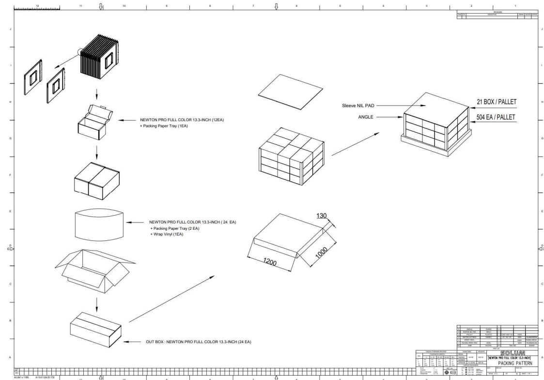
Figure 16. 13.3" Packing-Diagram (1,200 X 1,000)
