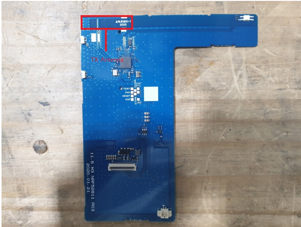
TX Antenna
