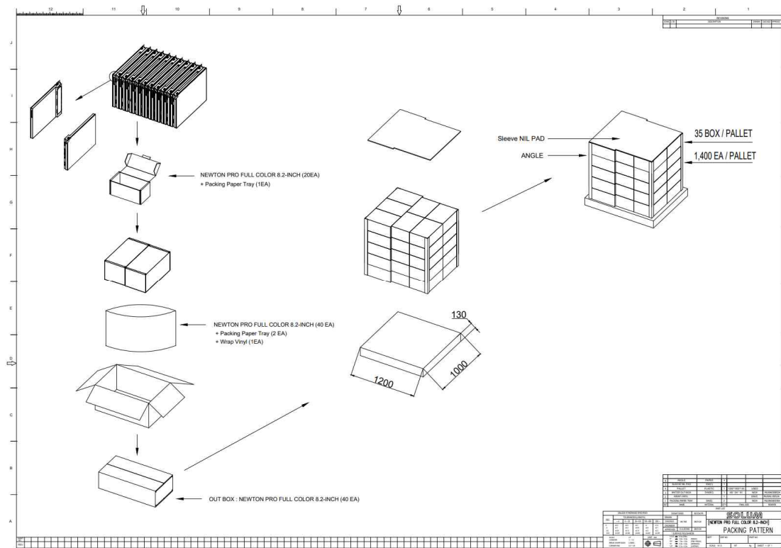
Figure 14. 8.2" Packing-Diagram (1,200 X 1,000)
