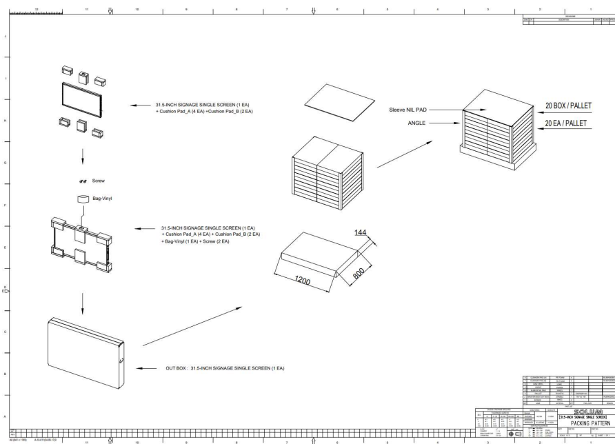
Figure 6. PACKING-DIAGRAM (1,200 X 800)
