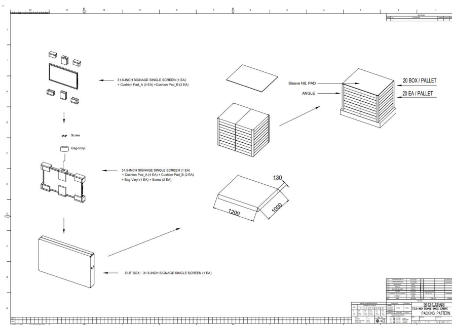
Figure 7. PACKING-DIAGRAM (1,200 X 1,000)
