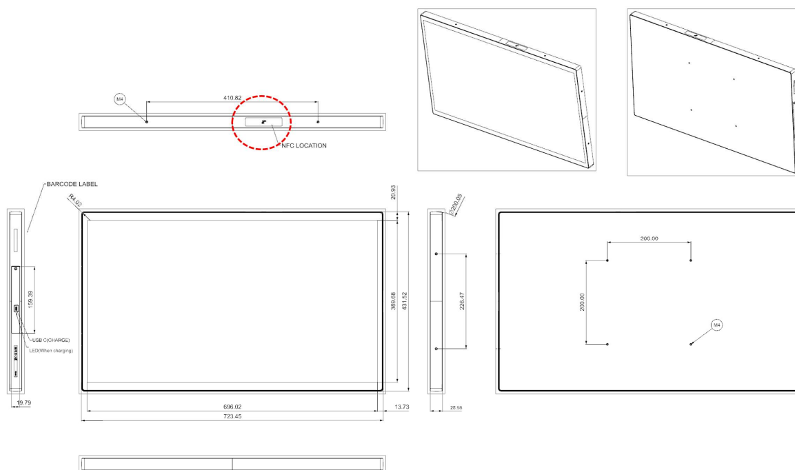
Figure 2. NFC LOCATION
