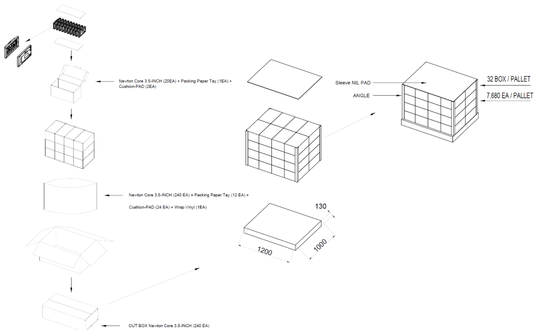
Figure 7. 3.5" Packing-Diagram (1,200 X 1,000)
