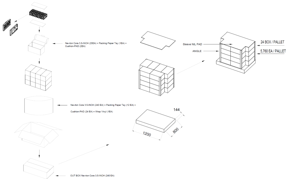
Figure 6. 3.5" Packing-Diagram (1,200 X 800)
