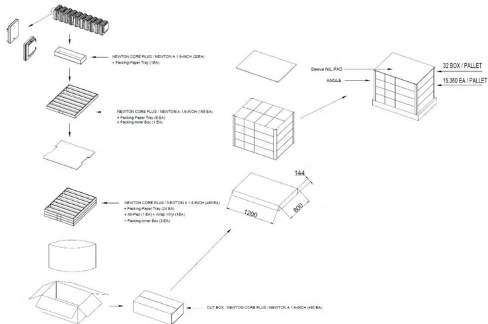
Figure 14. 1.6" PACKING-DIAGRAM (1,200 X 800)
