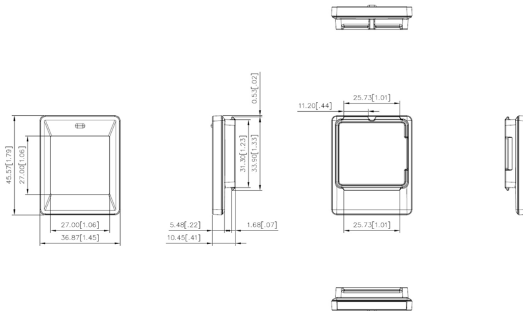
Figure 3. 1.6" MECHANICAL DIMENSION
