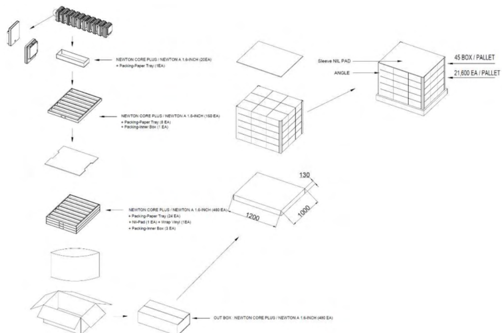
Figure 15. 1.6" PACKING-DIAGRAM (1,200 X 1,000)
