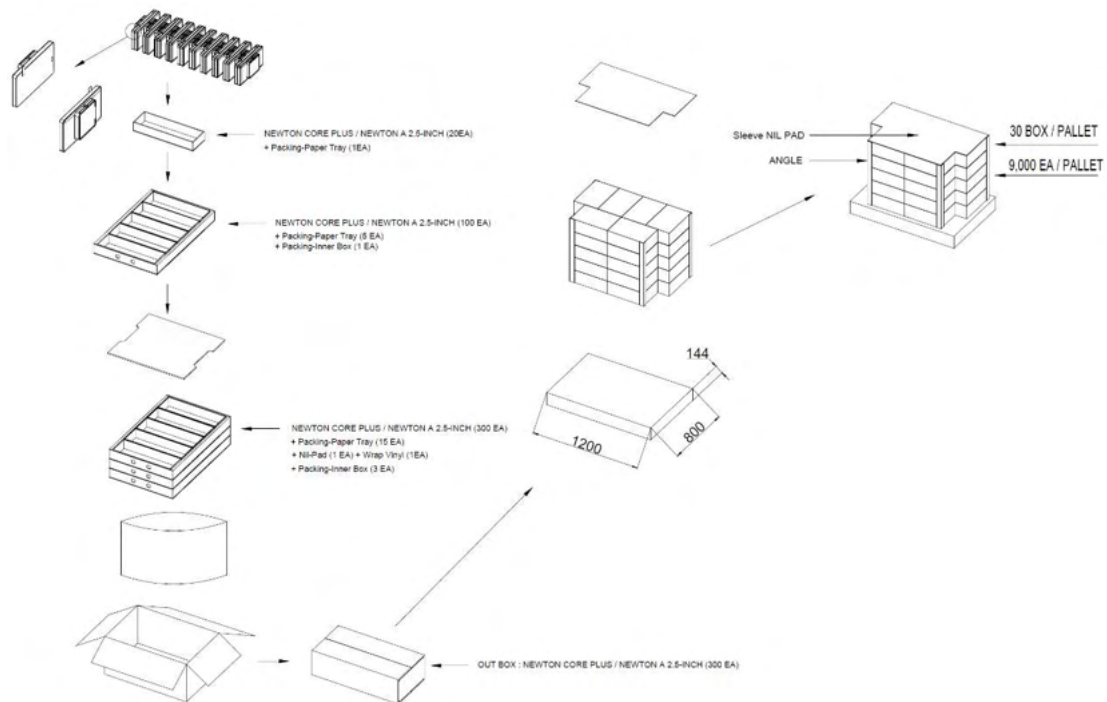
Figure 18. 2.5" PACKING-DIAGRAM (1,200 X 800)
