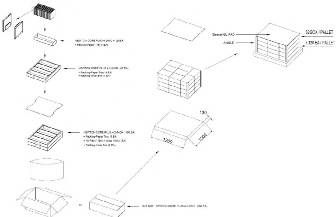
Figure 25. 4.2" PACKING-DIAGRAM (1,200 X 1,000)
