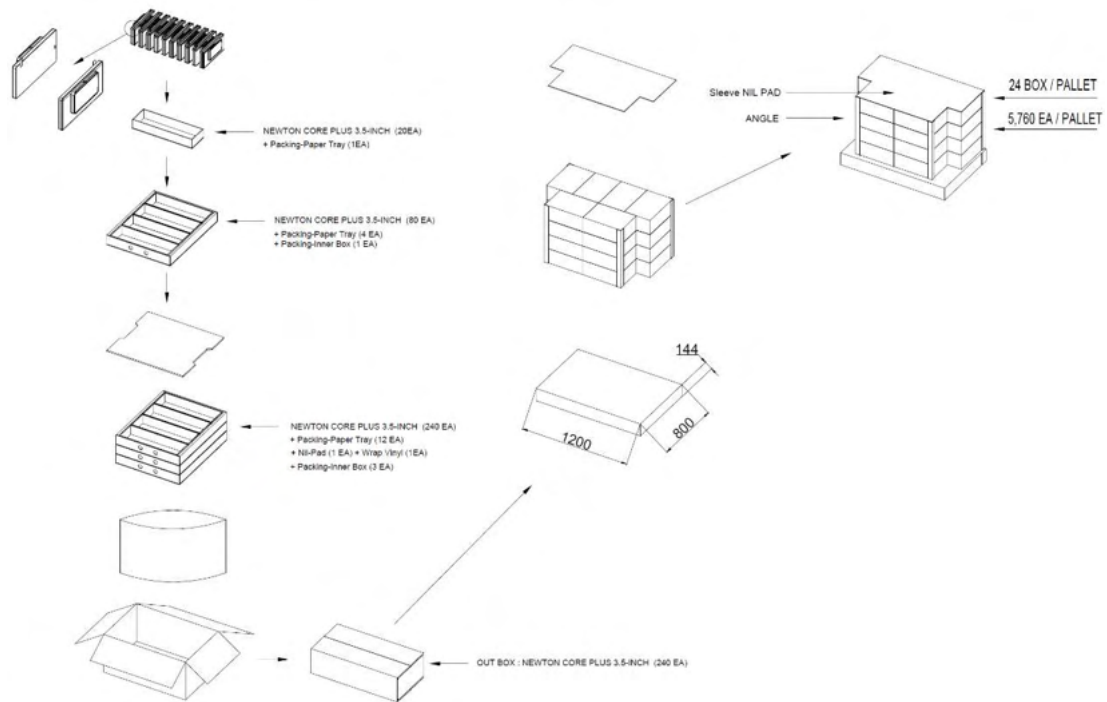
Figure 22. 3.5" PACKING-DIAGRAM (1,200 X 800)
