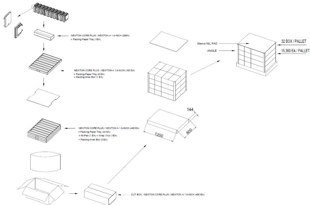
Figure 14. 1.6" PACKING-DIAGRAM (1,200 X 800)
