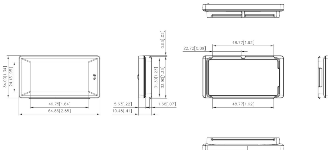
Figure 4. 2.1" MECHANICAL DIMENSION
