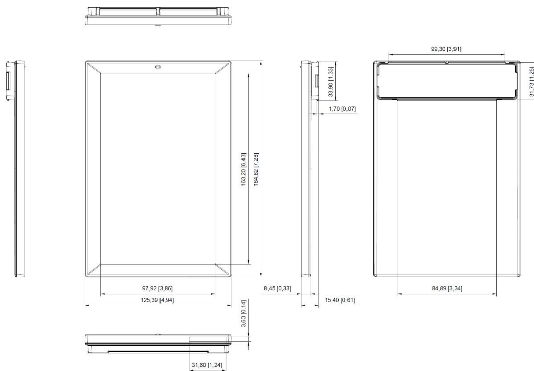
Figure 10. 7.5" MECHANICAL DIMENSION
