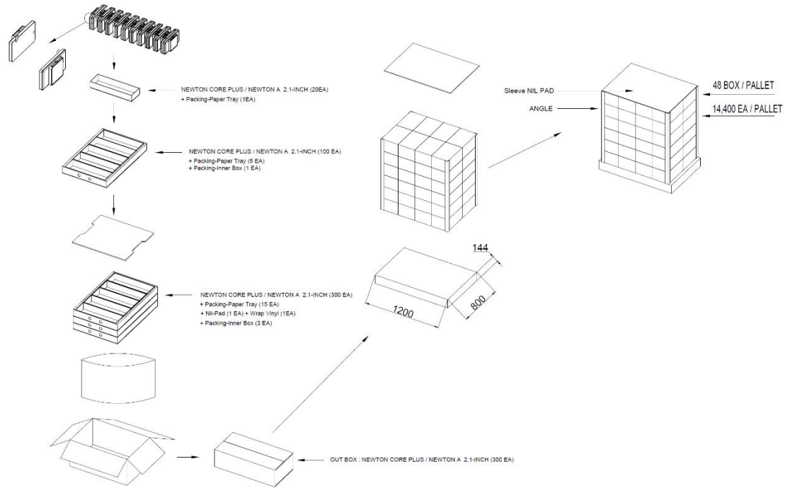
Figure 16. 2.1" PACKING-DIAGRAM (1,200 X 800)
