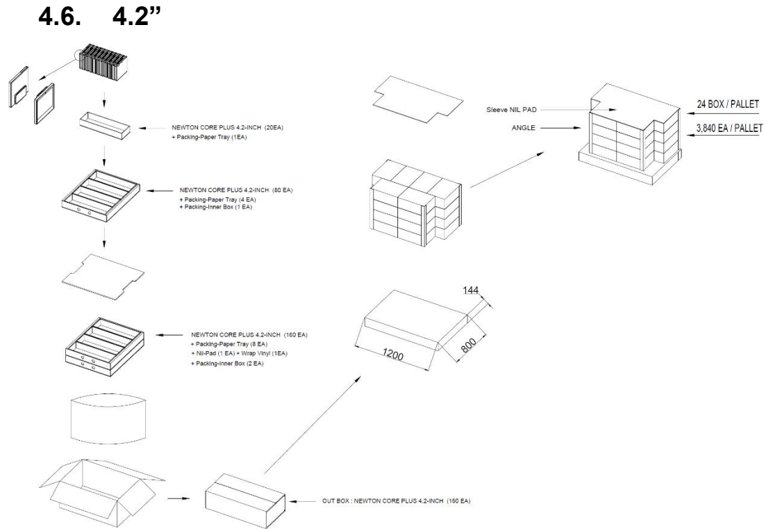
Figure 24. 4.2" PACKING-DIAGRAM (1,200 X 800)
