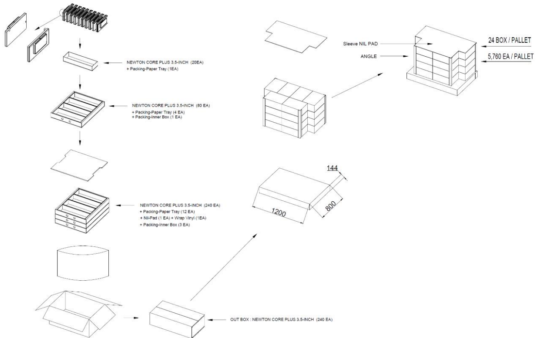
Figure 22. 3.5" PACKING-DIAGRAM (1,200 X 800)
