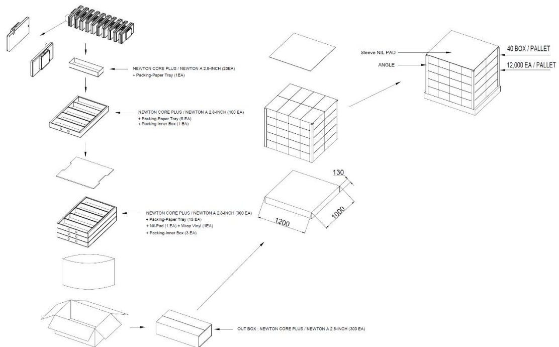
Figure 21. 2.8" PACKING-DIAGRAM (1,200 X 1,000)
