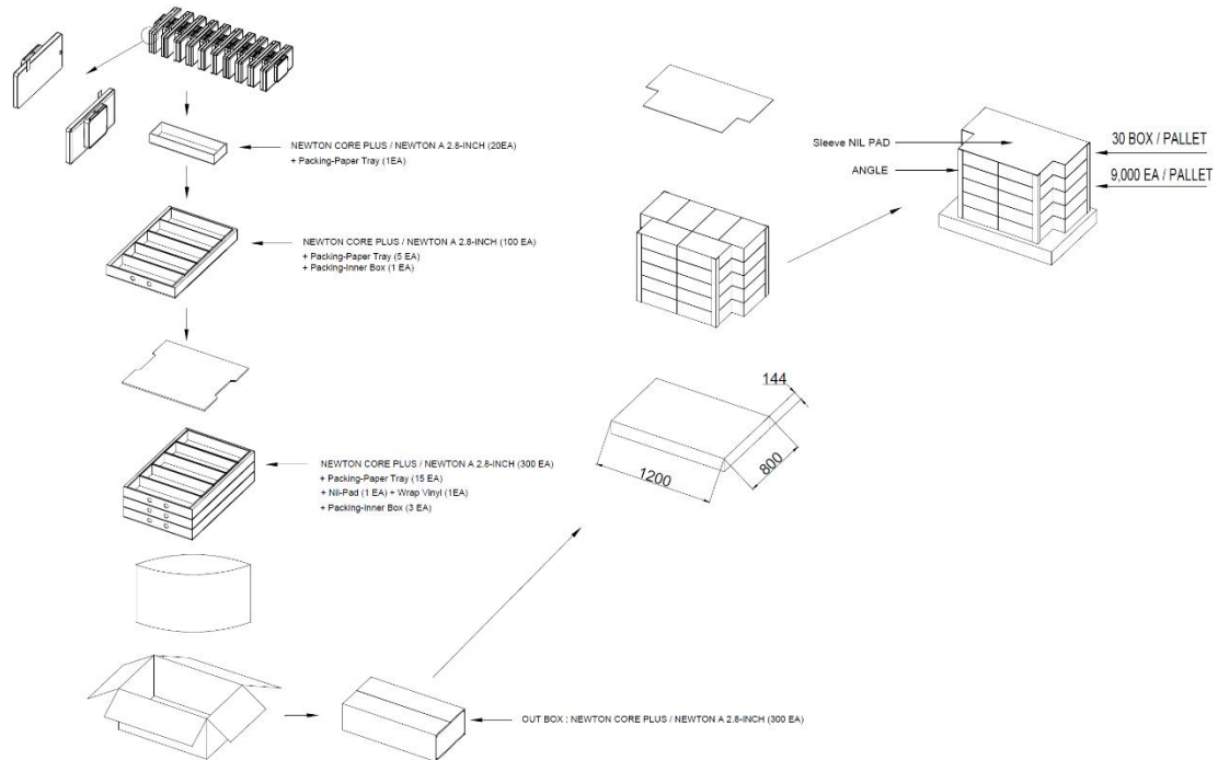
Figure 20. 2.8" PACKING-DIAGRAM (1,200 X 800)
