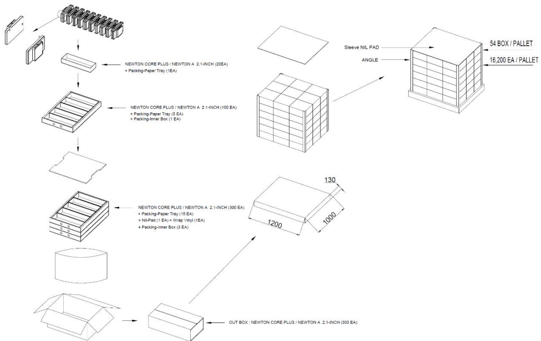
Figure 17. 2.1" PACKING-DIAGRAM (1,200 X 1,000)
