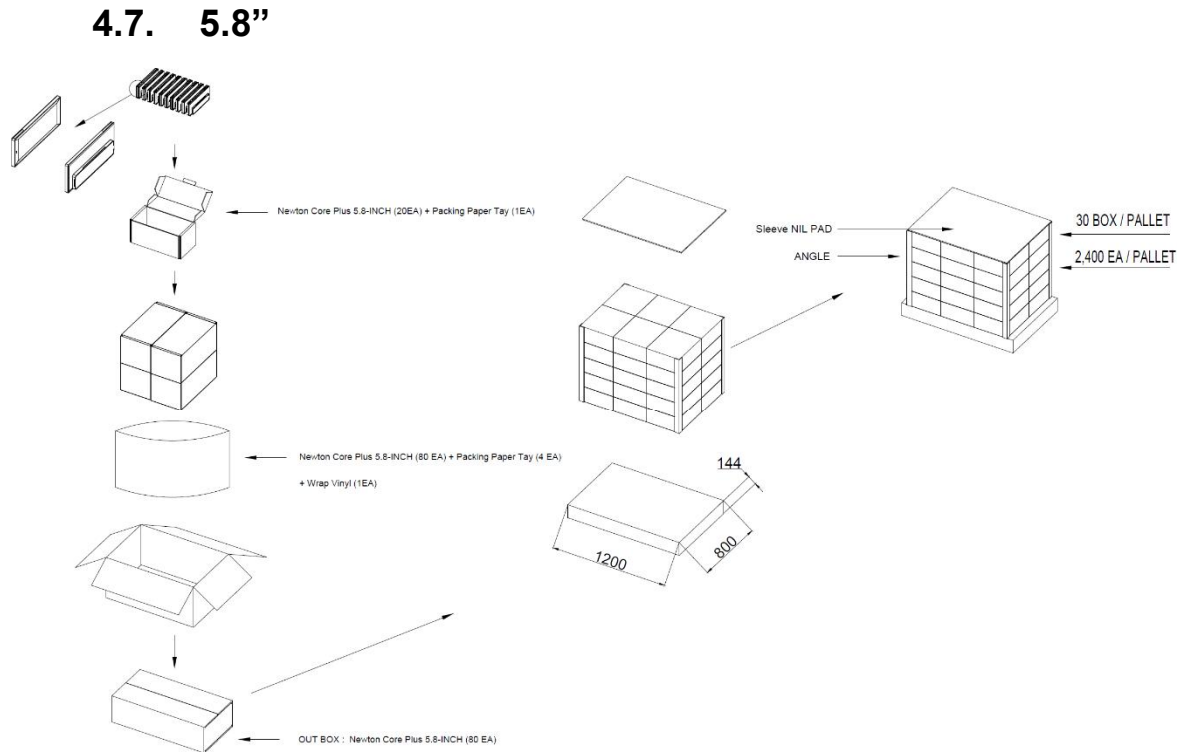
Figure 26. 5.8" PACKING-DIAGRAM (1,200 X 800)
