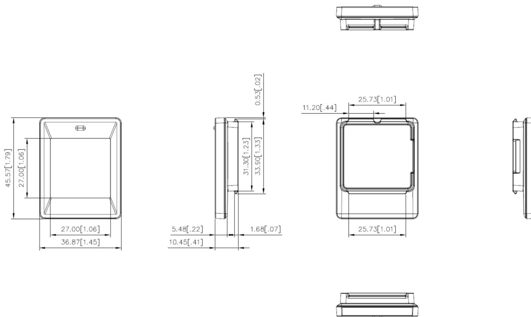
Figure 3. 1.6" MECHANICAL DIMENSION
