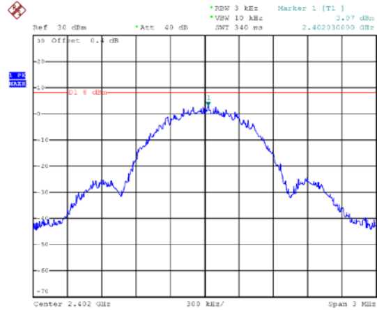
Test Mode : ANT2 Low channel
