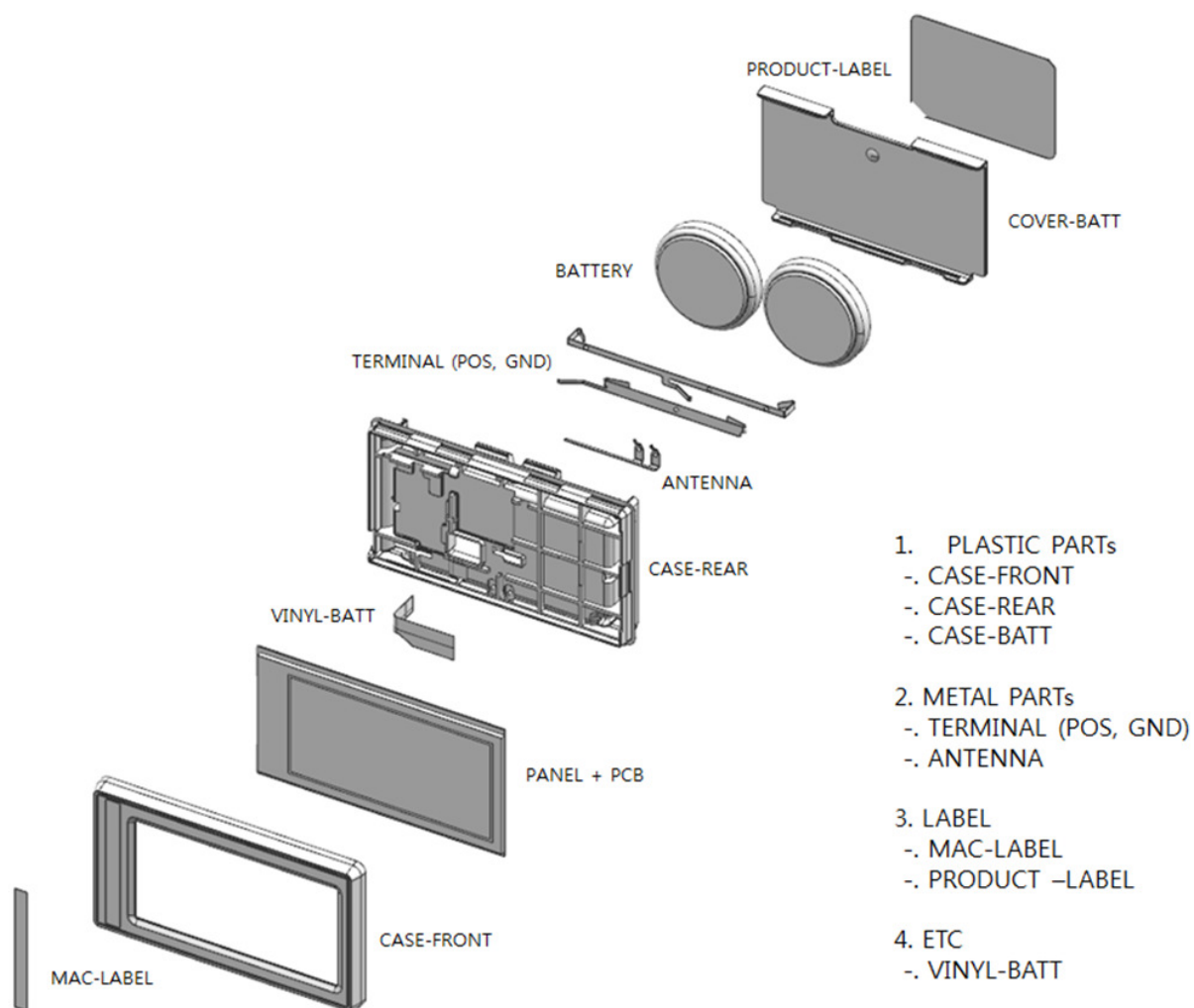
Figure 4 Exploded View
