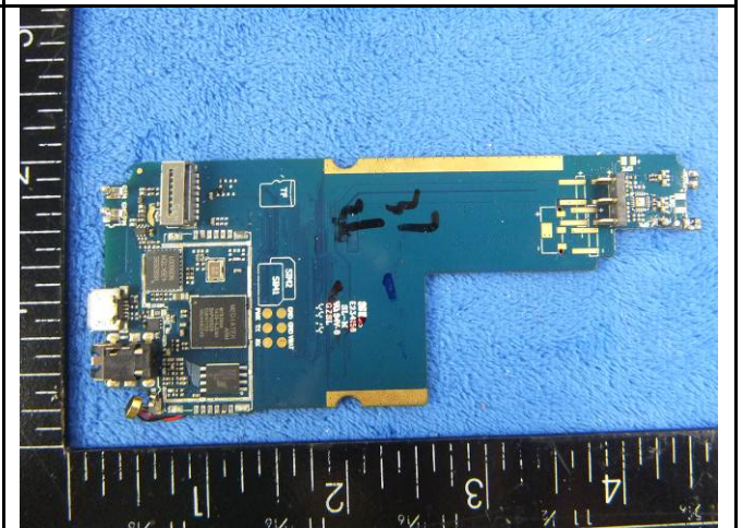
Mainboard with Shielding – Front View
