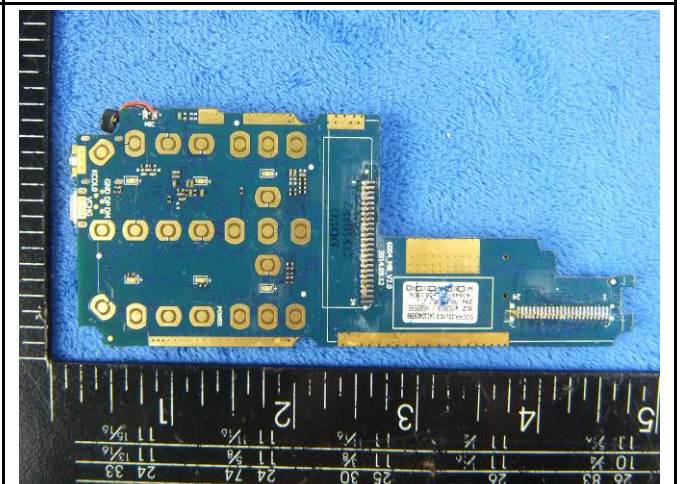
Mainboard without Shielding - Rear View
