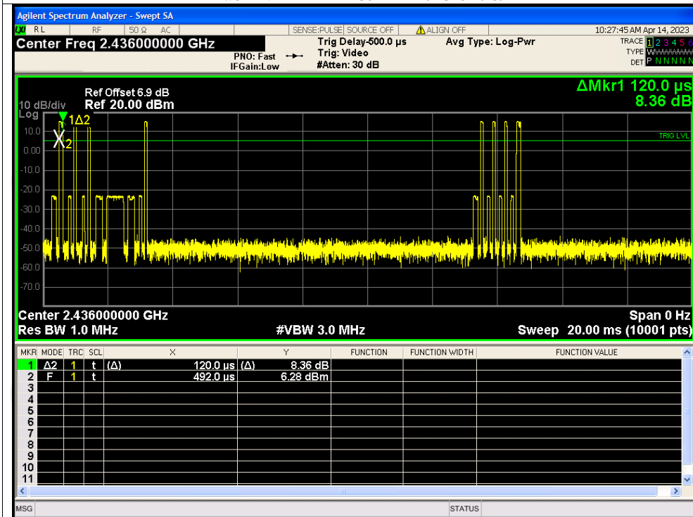
Dwell NVNT 1-DH1 2436MHz Ant1 Accumulated
