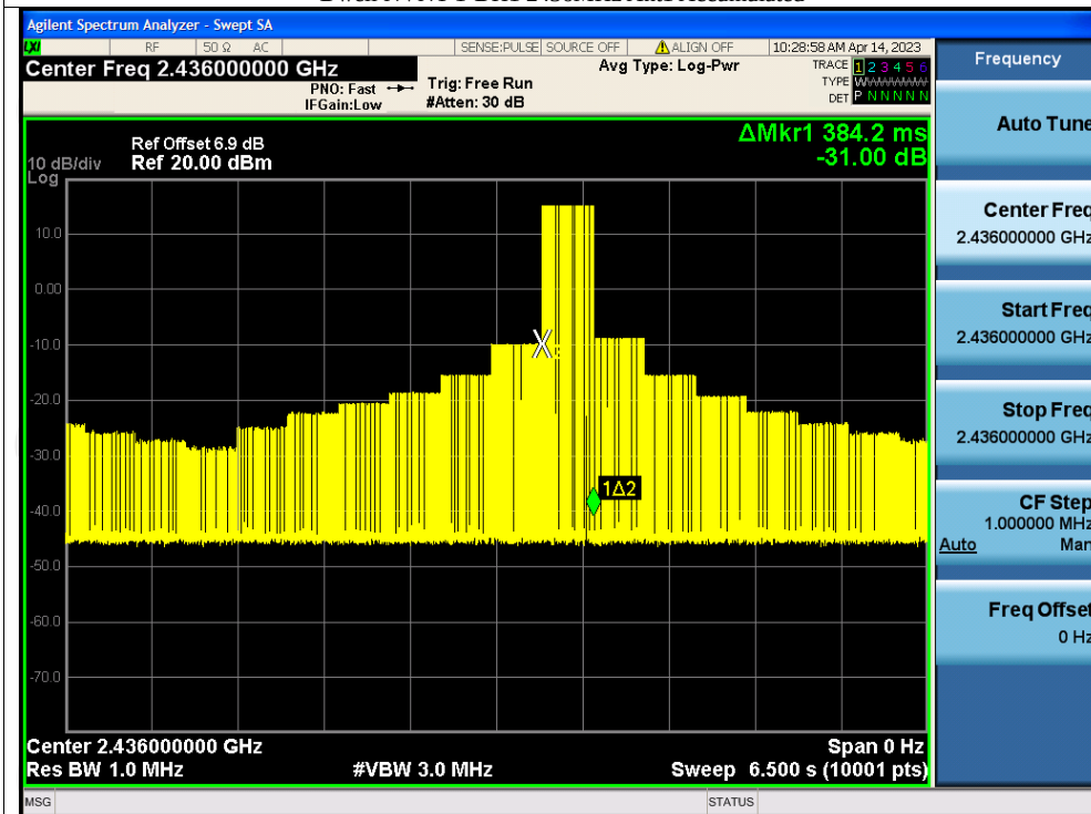
Dwell NVNT 2.4G 2436MHz Accumulated
