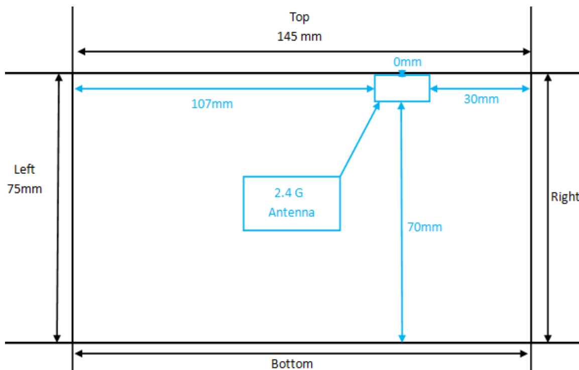
Antenna Configuration 1- Vertical ( Antenna is unfolded and is Vertical to the edge of EUT )
