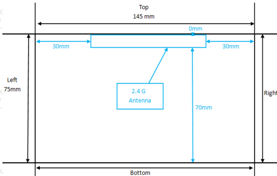
Antenna Configuration 1-Level ( Antenna is folded and align with the edge of EUT )
